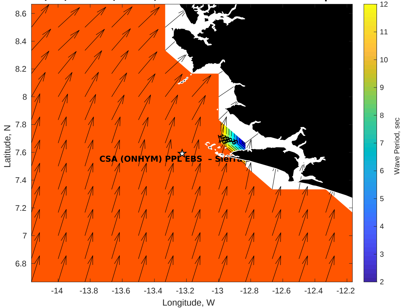
Wave Period (sec) for CSA (ONHYM) PPL EBS - Sierra Leone at 07-Sep-2025 09:00:00
