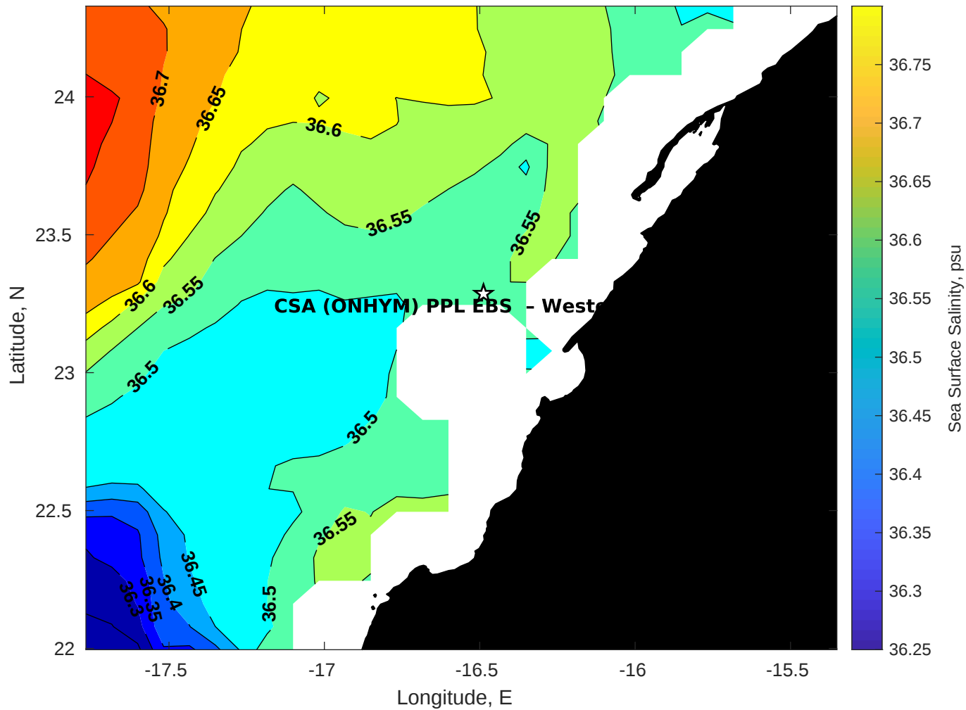
Surface Salinity for CSA (ONHYM) PPL EBS - Western Sahara at 06-Sep-2025 00:00:00
