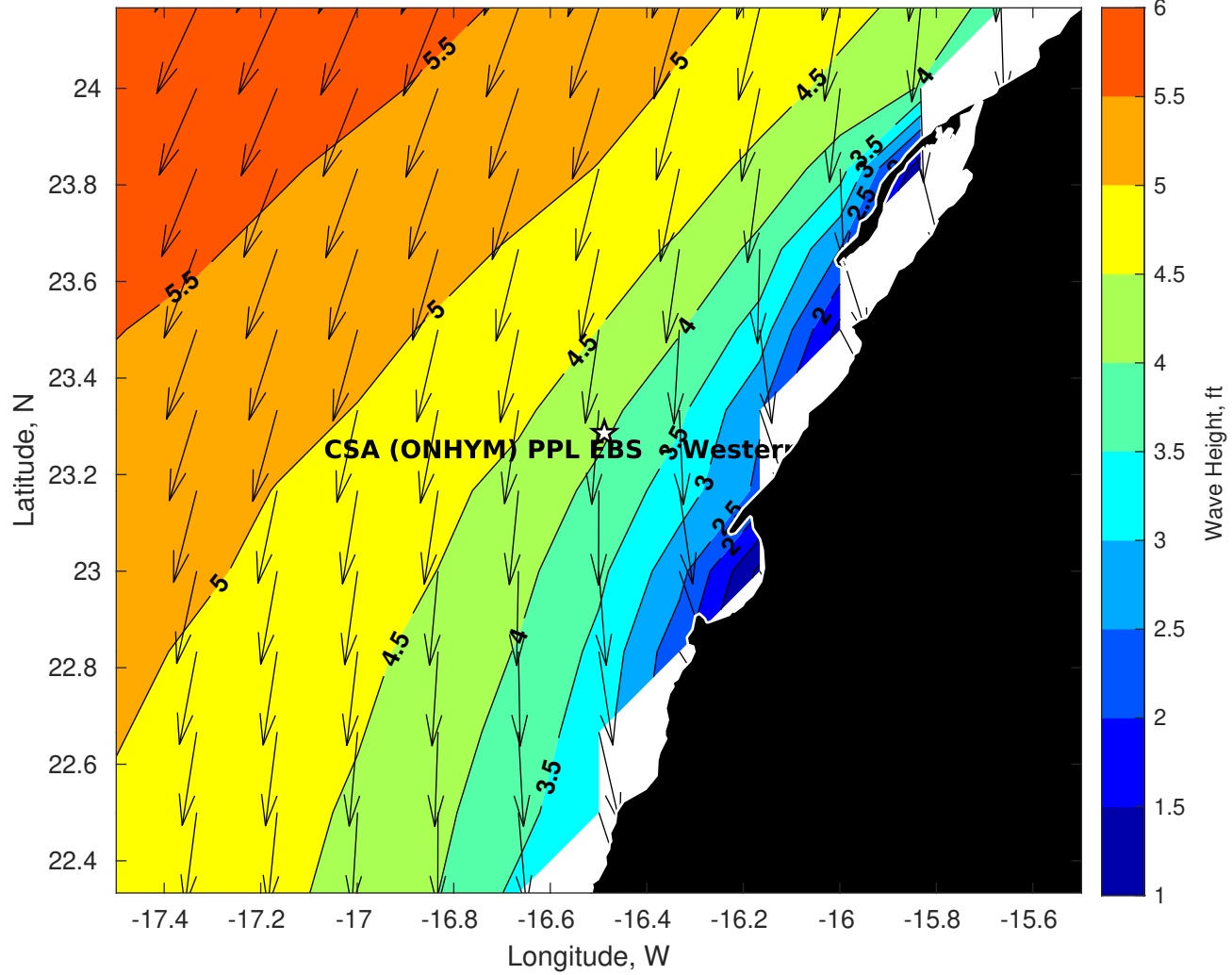
Wave Height (ft) for CSA (ONHYM) PPL EBS - Western Sahara at 07-Sep-2025 09:00:00
