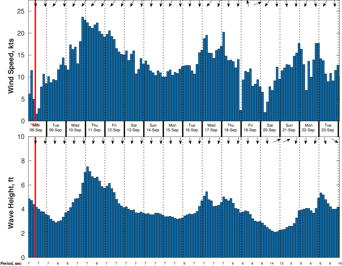
Wind & Wave Forecast for CSA (ONHYM) PPL EBS - Western Sahara from 07-Sep-2025 01:00:00 to 23-Sep-2025 01:00:00
