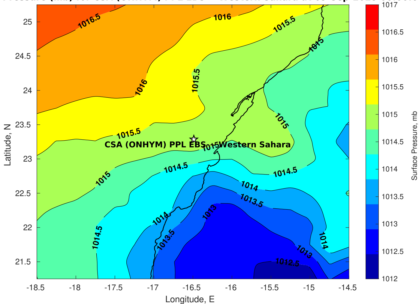
Surface Pressure (mb) for CSA (ONHYM) PPL EBS - Western Sahara at 09-Sep-2025 00:00:00
