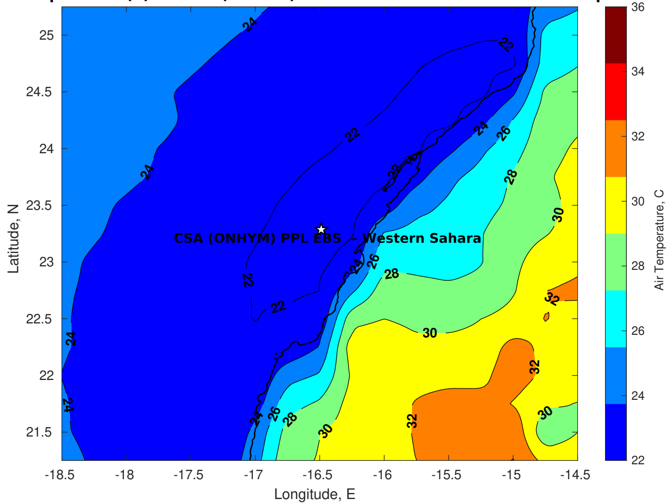
Air Temperature (C) for CSA (ONHYM) PPL EBS - Western Sahara at 07-Sep-2025
