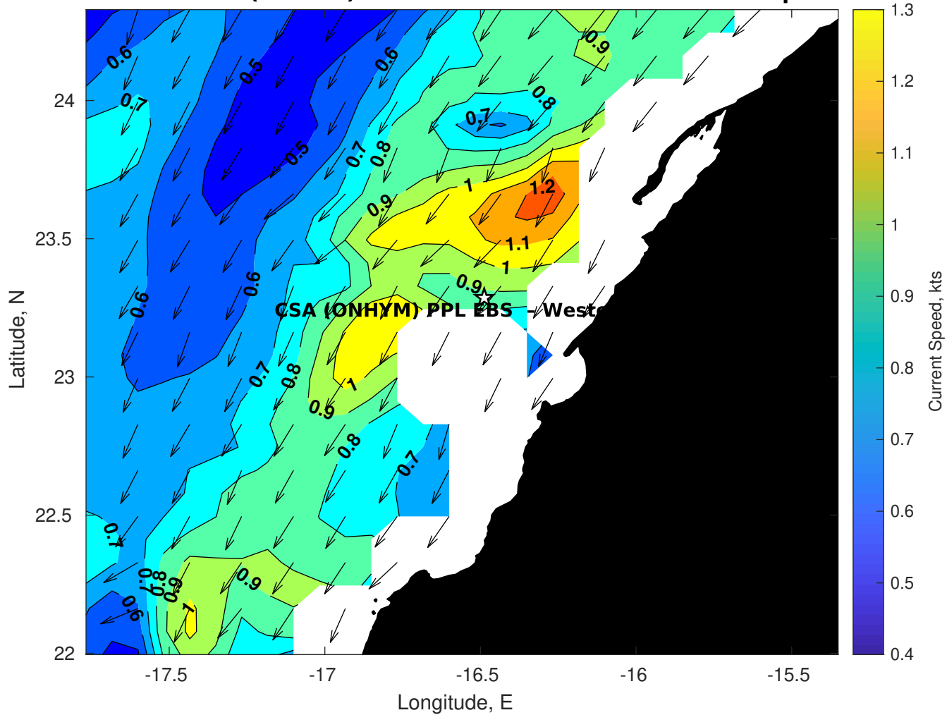
Surface Currents for CSA (ONHYM) PPL EBS - Western Sahara at 06-Sep-2025 00:00:00
