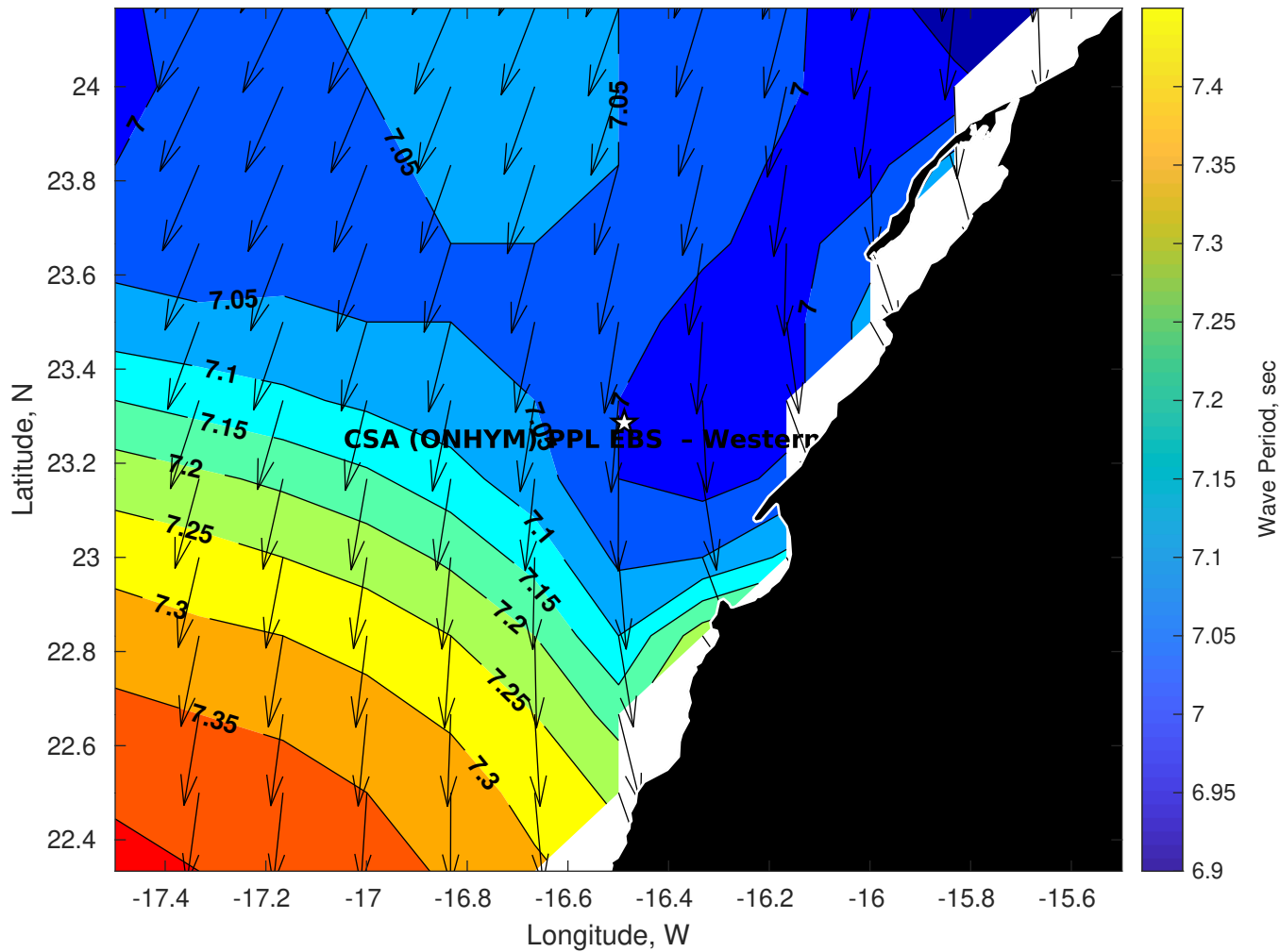
Wave Period (sec) for CSA (ONHYM) PPL EBS - Western Sahara at 07-Sep-2025 09:00:00
