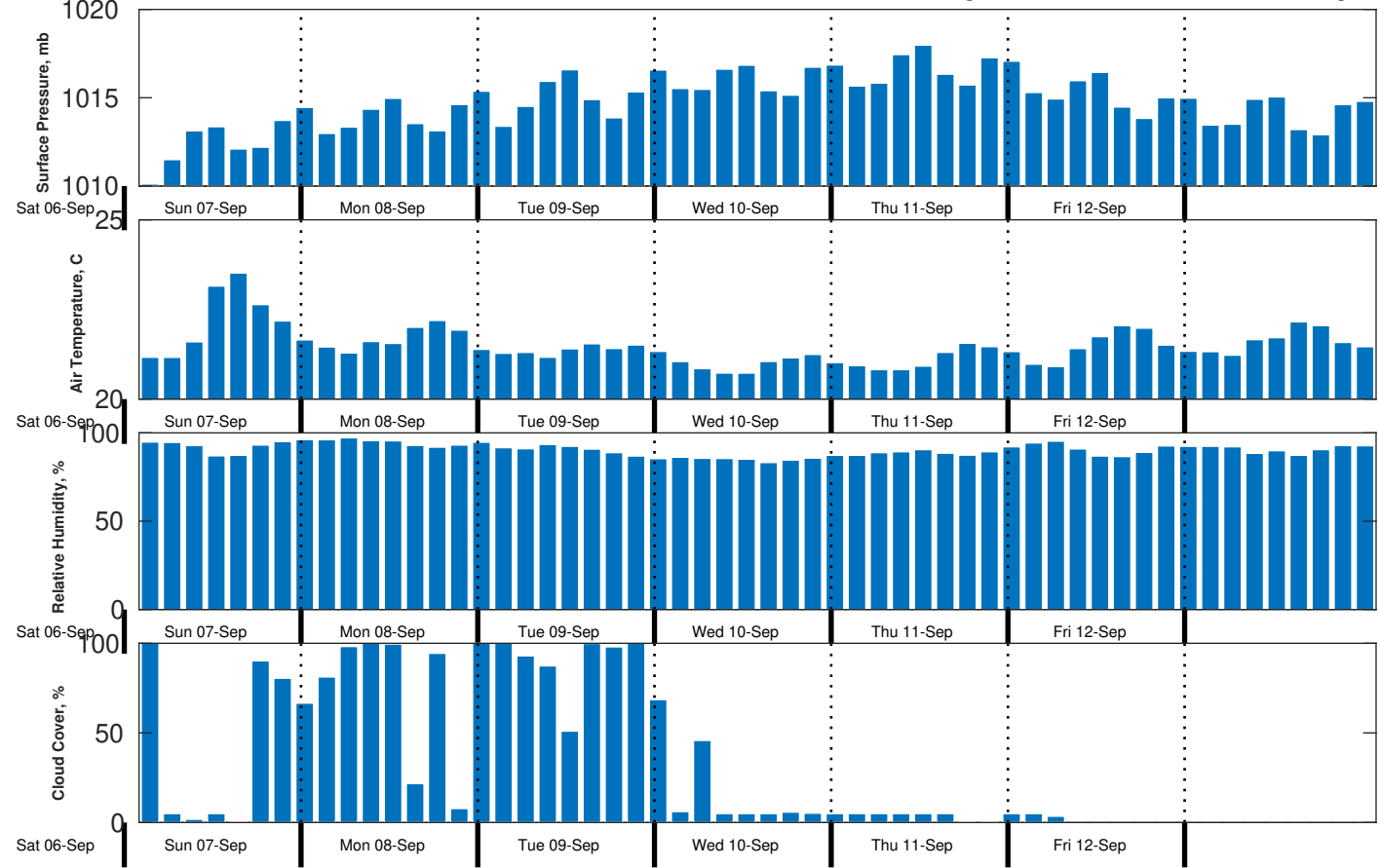
Met Forecast for CSA (ONHYM) PPL EBS - Western Sahara from 07-Sep-2025 00:00:00 to 14-Sep-2025 00:00:00
