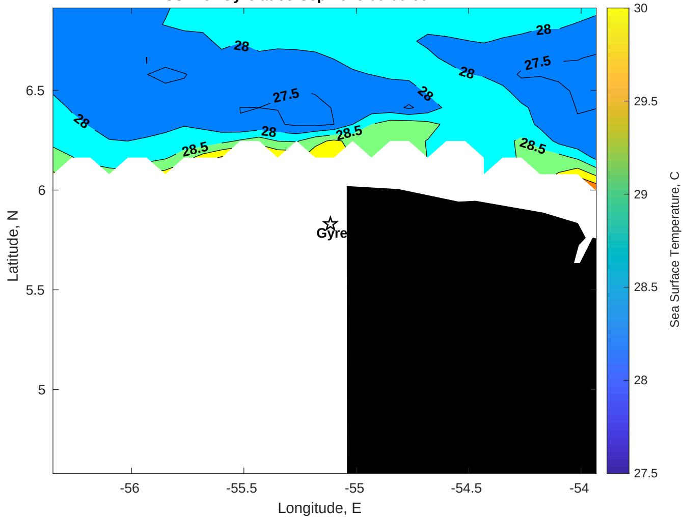
SST for Gyre at 06-Sep-2025 00:00:00
