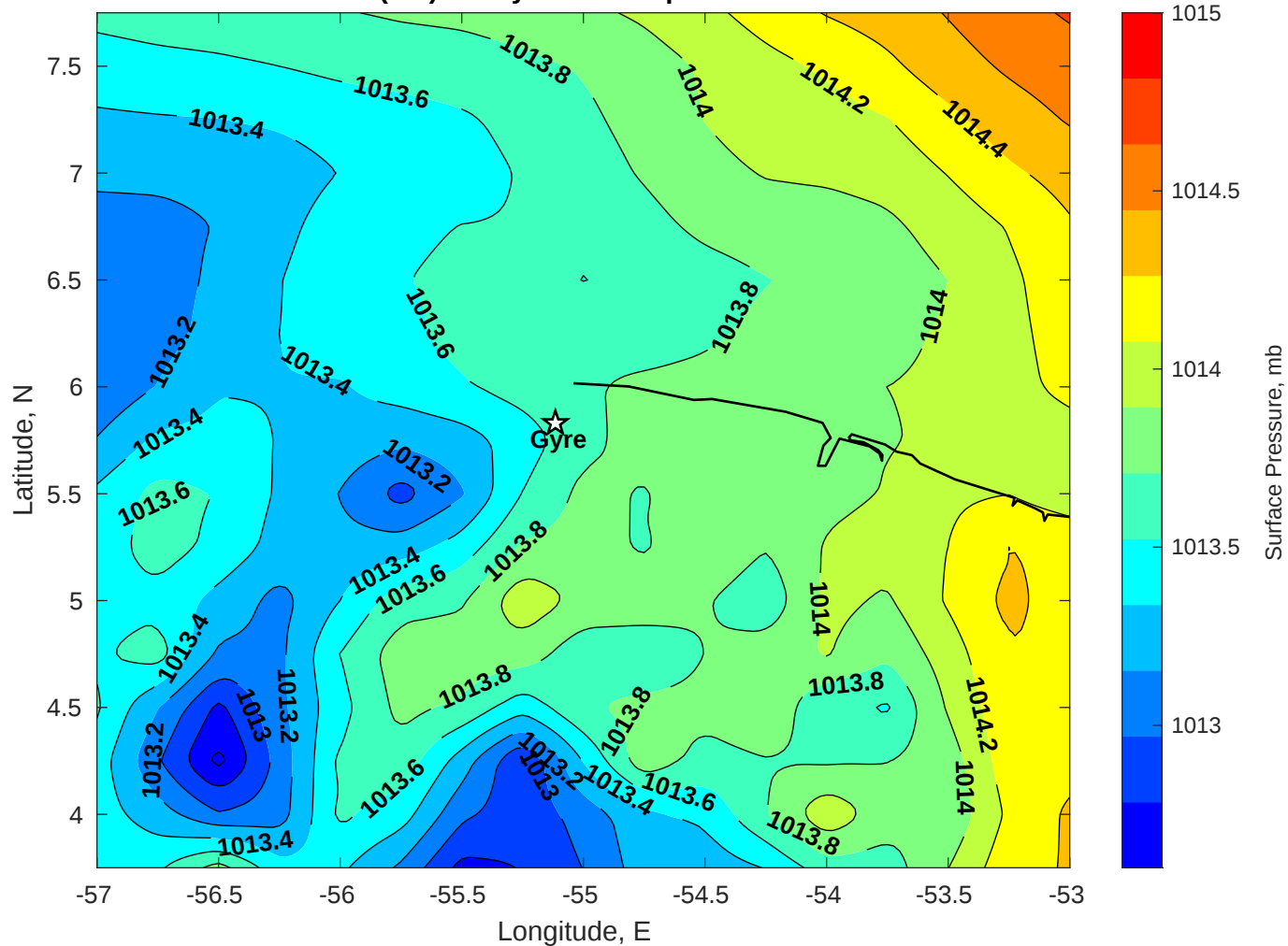
Surface Pressure (mb) for Gyre at 08-Sep-2025 00:00:00
