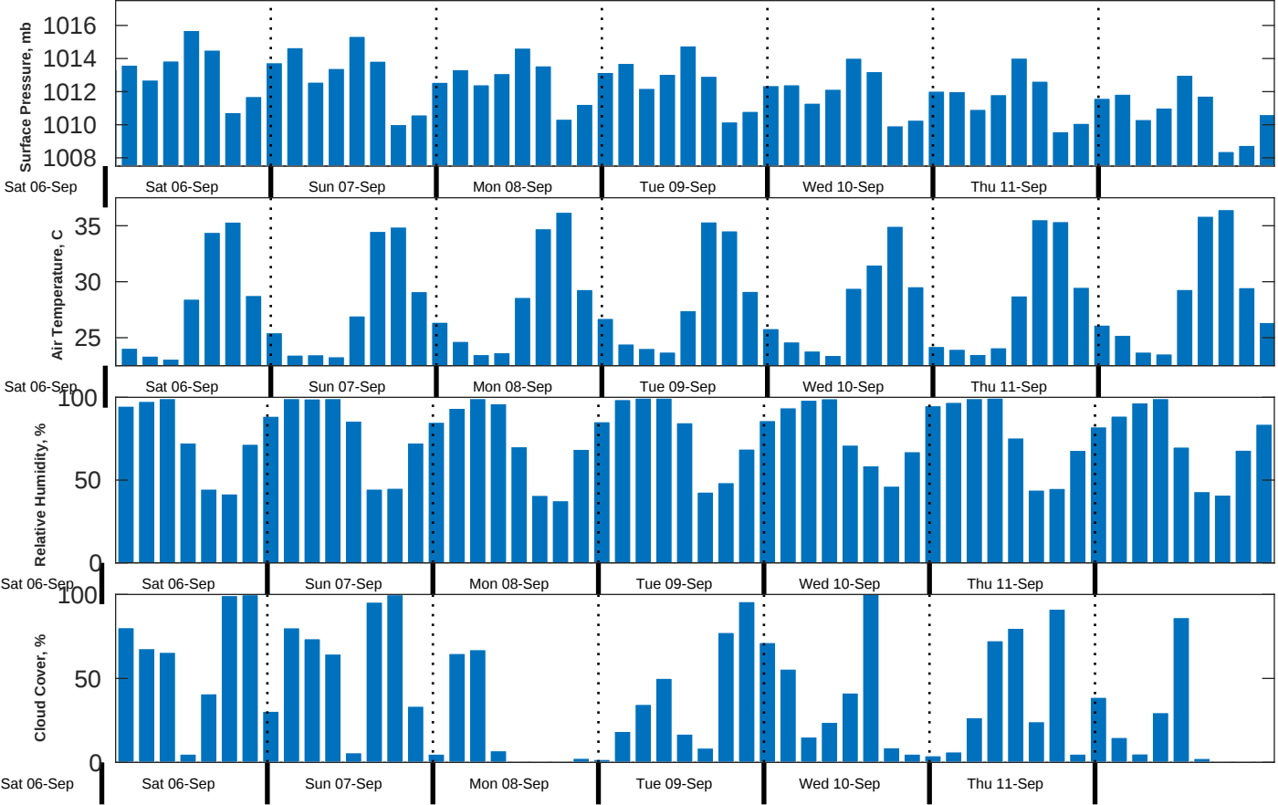
Met Forecast for Gyre from 06-Sep-2025 20:00:00 to 13-Sep-2025 20:00:00
