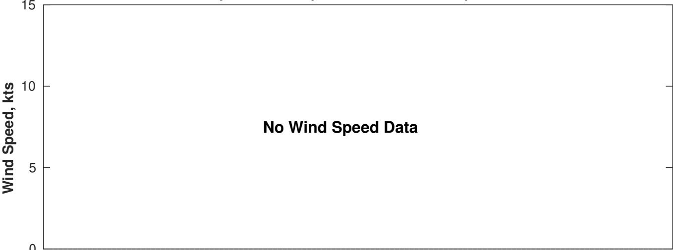
Wind & Wave Forecast for Gyre from 06-Sep-2025 20:00:00 to 22-Sep-2025 20:00:00
