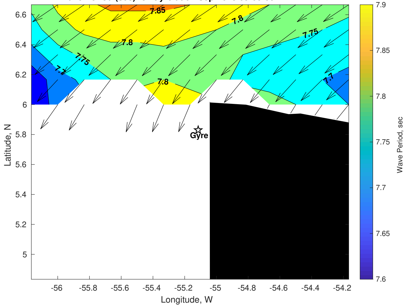
Wave Period (sec) for Gyre at 07-Sep-2025 09:00:00
