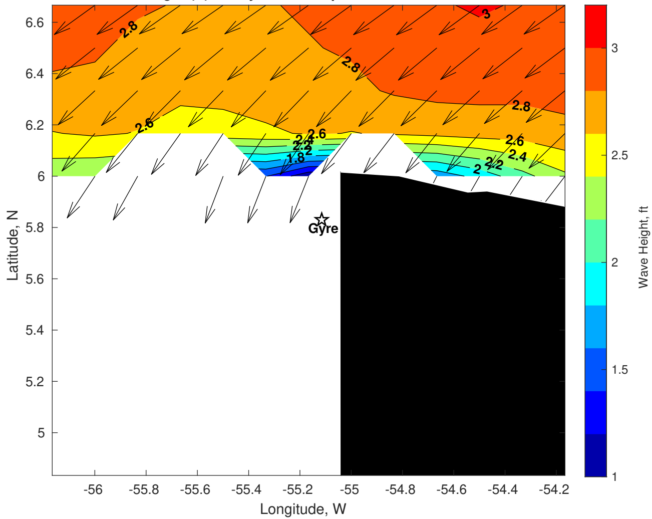
Wave Height (ft) for Gyre at 07-Sep-2025 09:00:00
