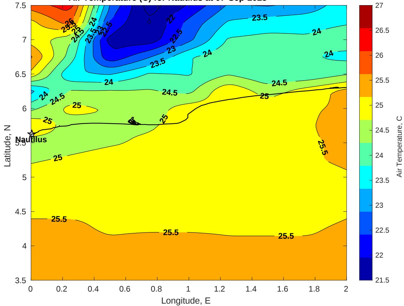
Air Temperature (C) for Nautilus at 07-Sep-2025
