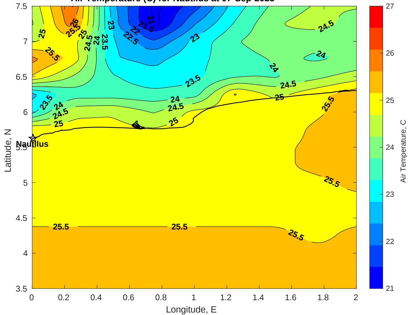
Air Temperature (C) for Nautilus at 07-Sep-2025
