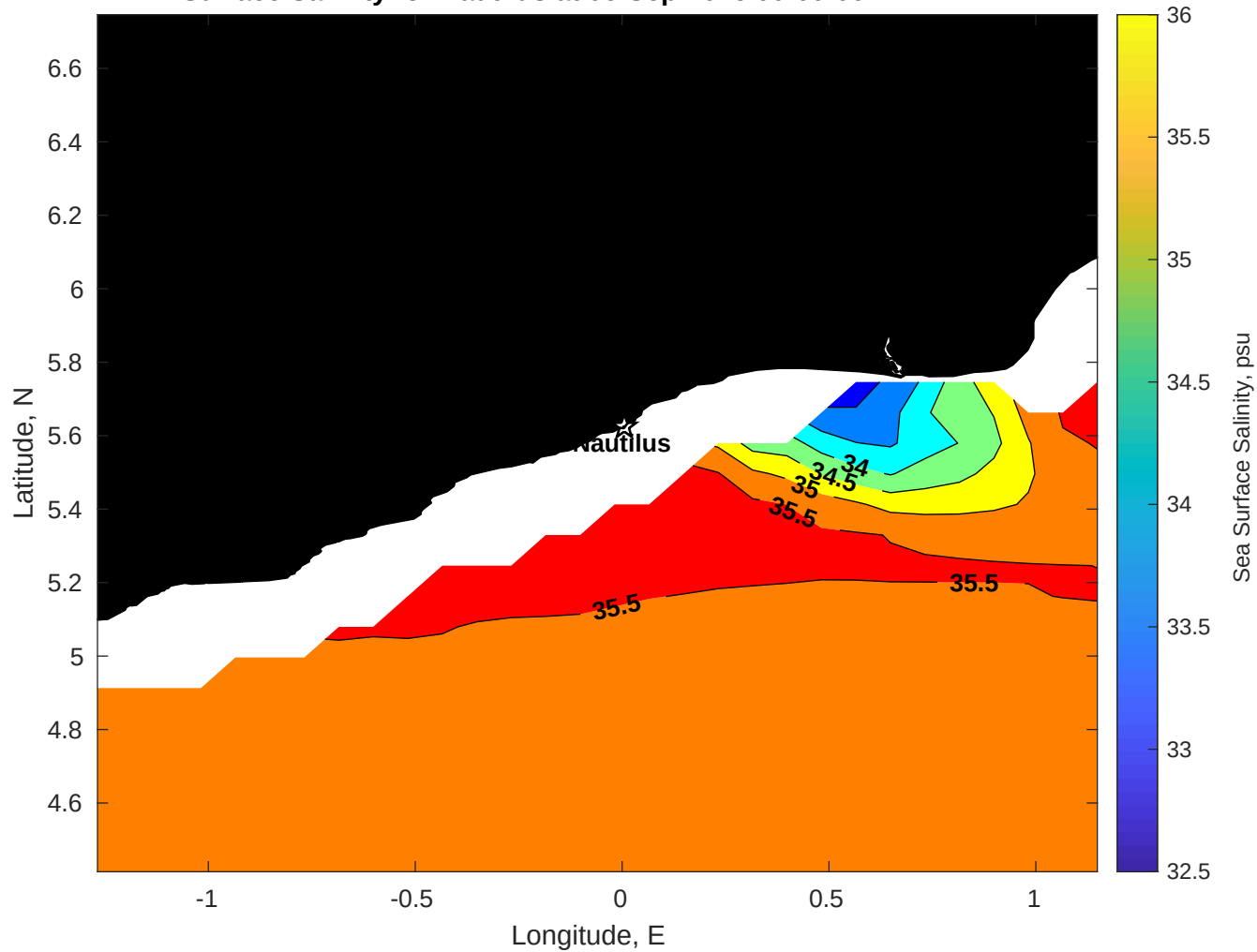
Surface Salinity for Nautilus at 06-Sep-2025 00:00:00
