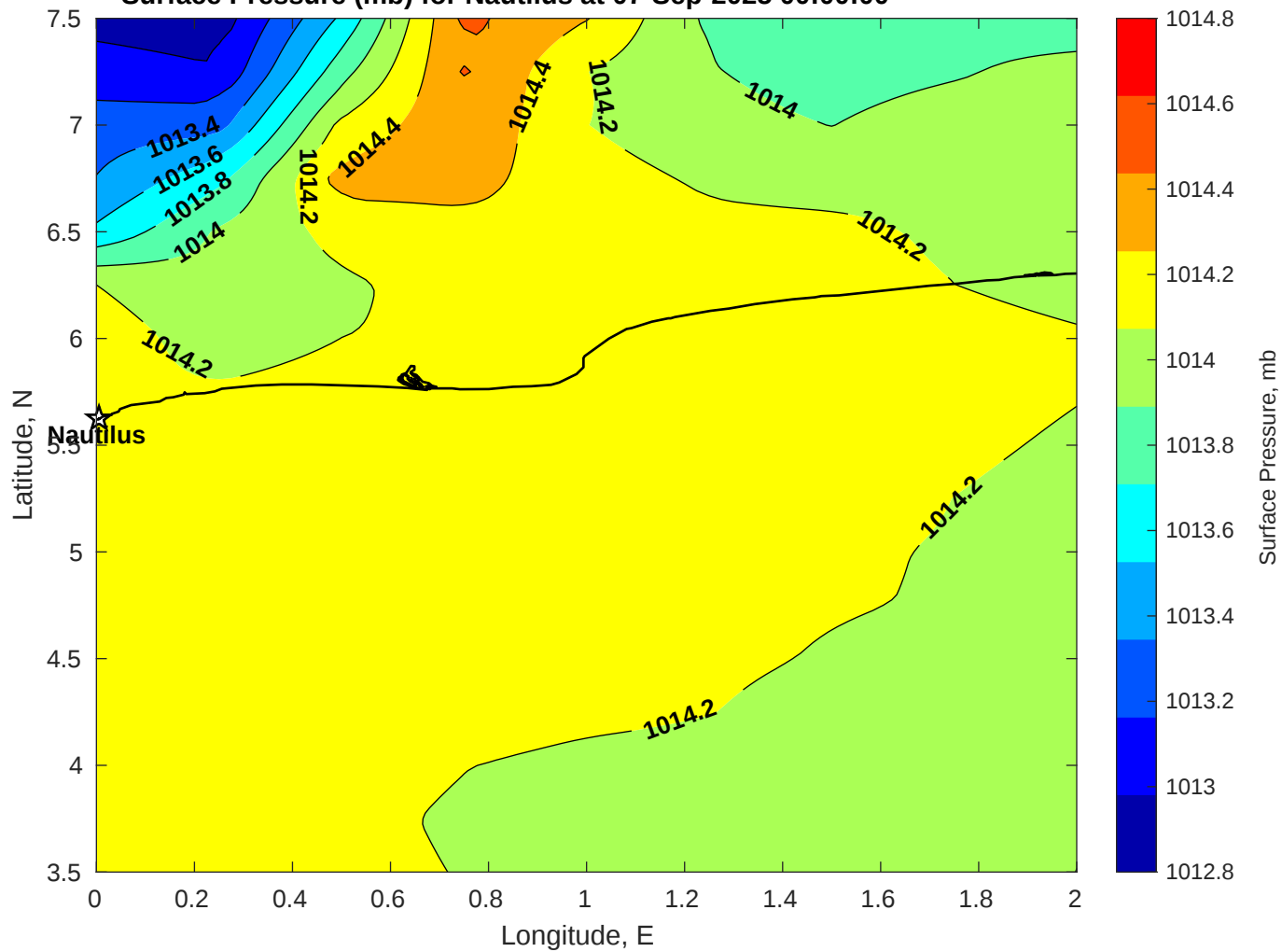
Surface Pressure (mb) for Nautilus at 07-Sep-2025 00:00:00
