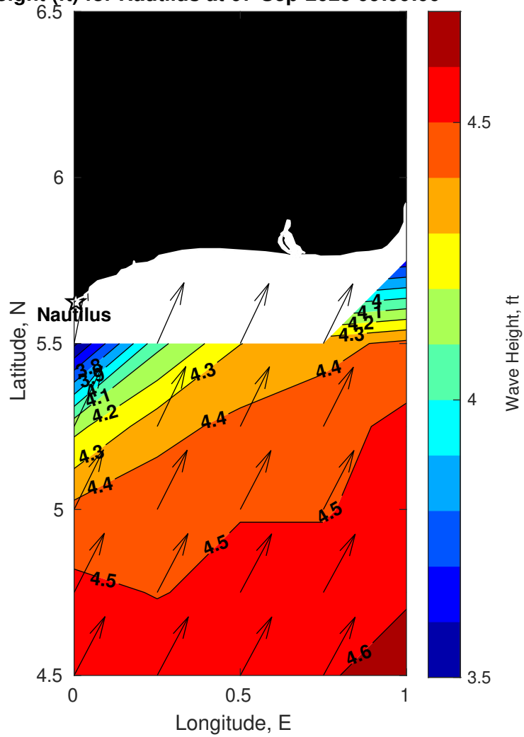
Wave Height (ft) for Nautilus at 07-Sep-2025 09:00:00
