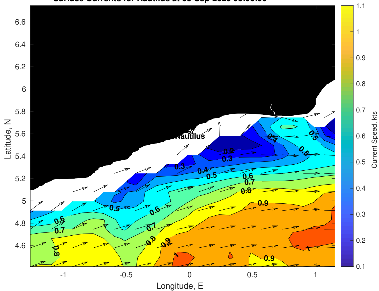
Surface Currents for Nautilus at 06-Sep-2025 00:00:00
