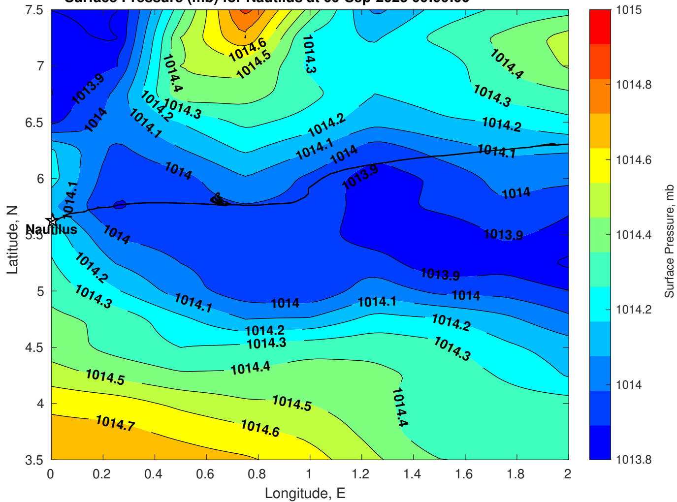
Surface Pressure (mb) for Nautilus at 09-Sep-2025 00:00:00
