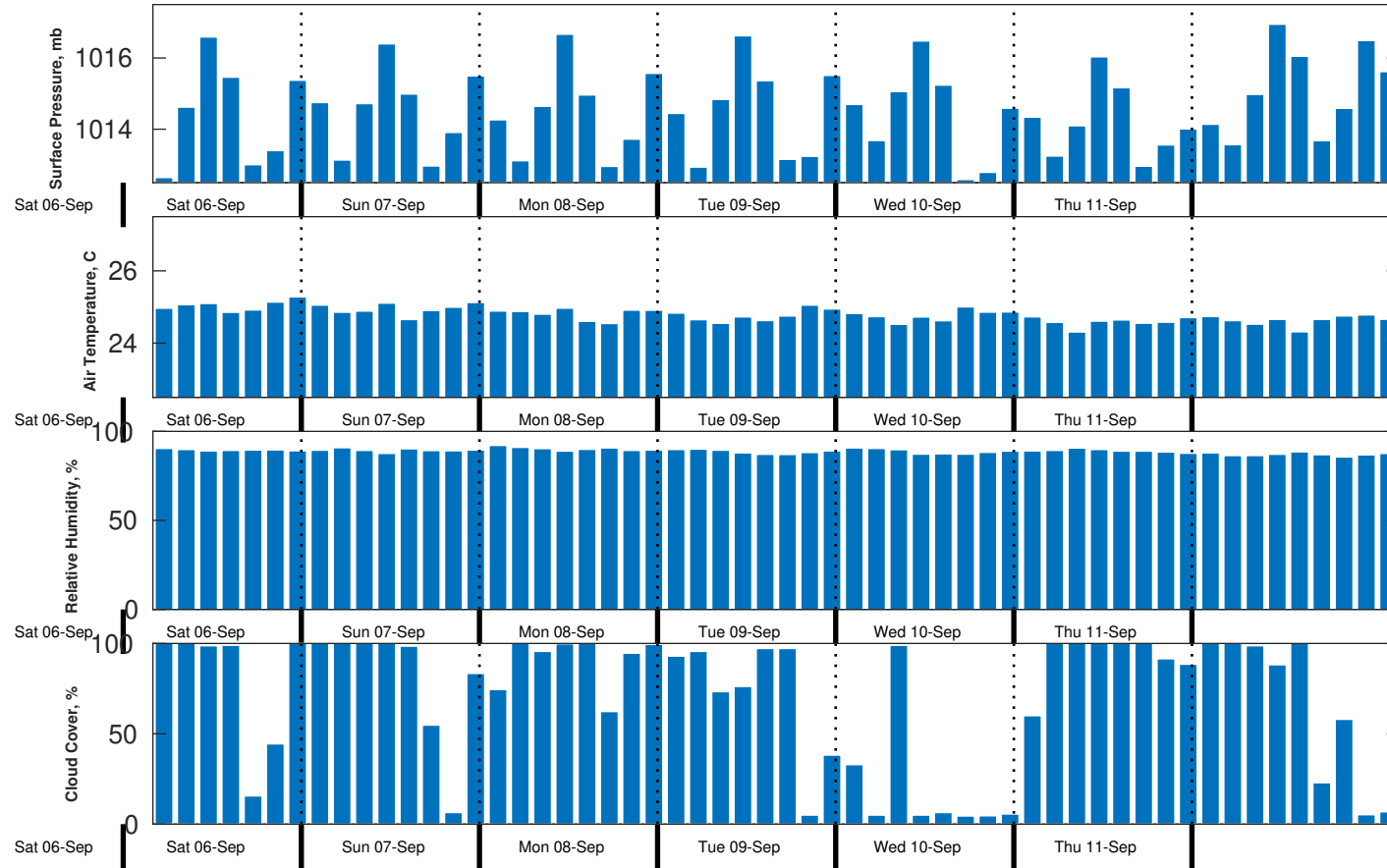
Met Forecast for Nautilus from 07-Sep-2025 00:00:00 to 14-Sep-2025 00:00:00
