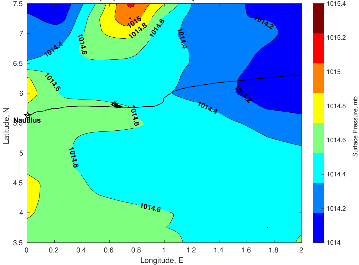
Surface Pressure (mb) for Nautilus at 08-Sep-2025 00:00:00
