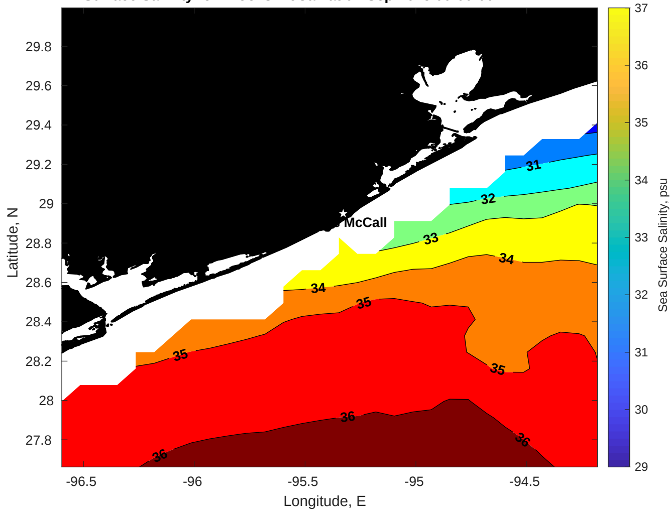
Surface Salinity for Brooks McCall at 07-Sep-2025 00:00:00
