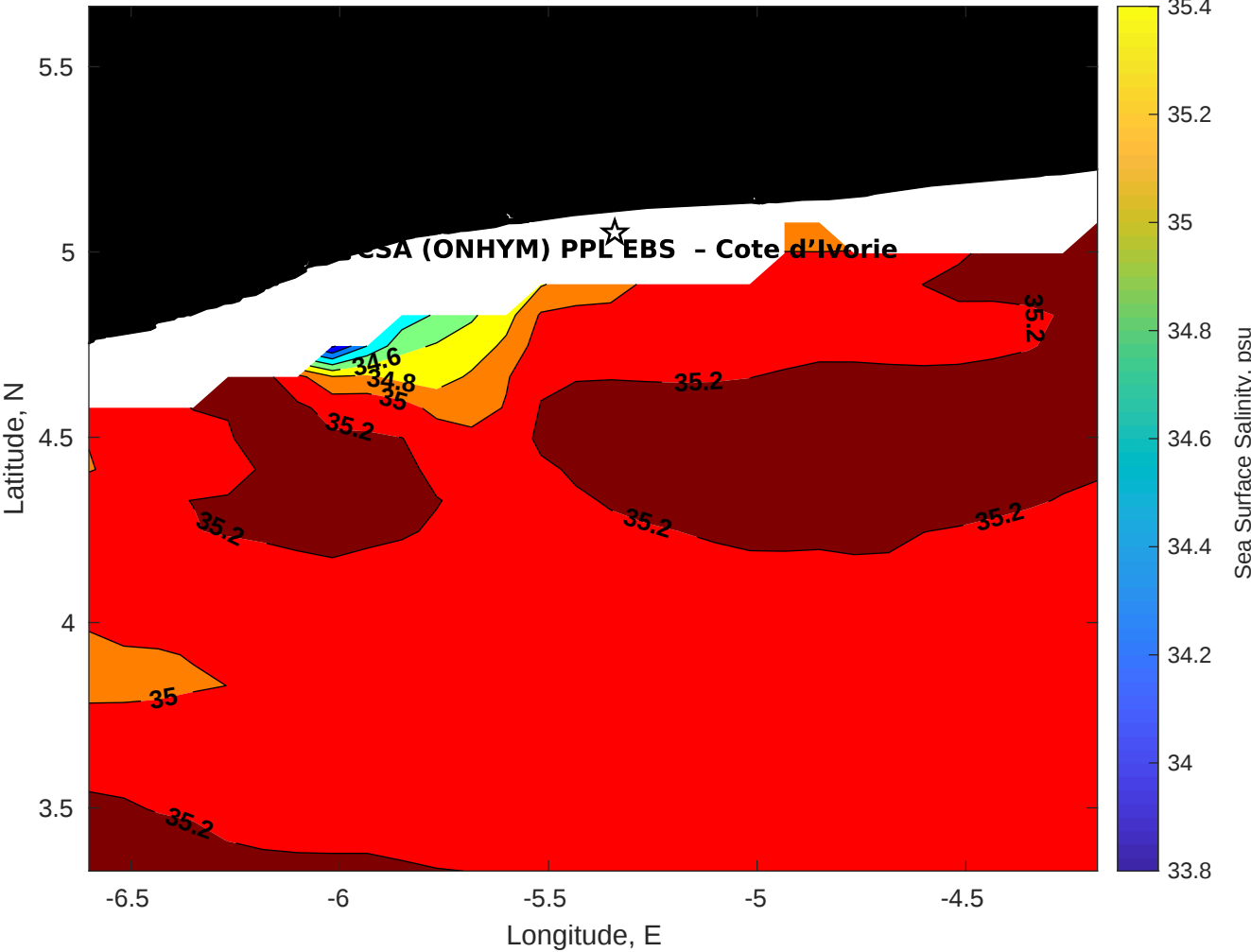
Surface Salinity for CSA (ONHYM) PPL EBS - Cote d'Ivoire at 07-Sep-2025 00:00:00
