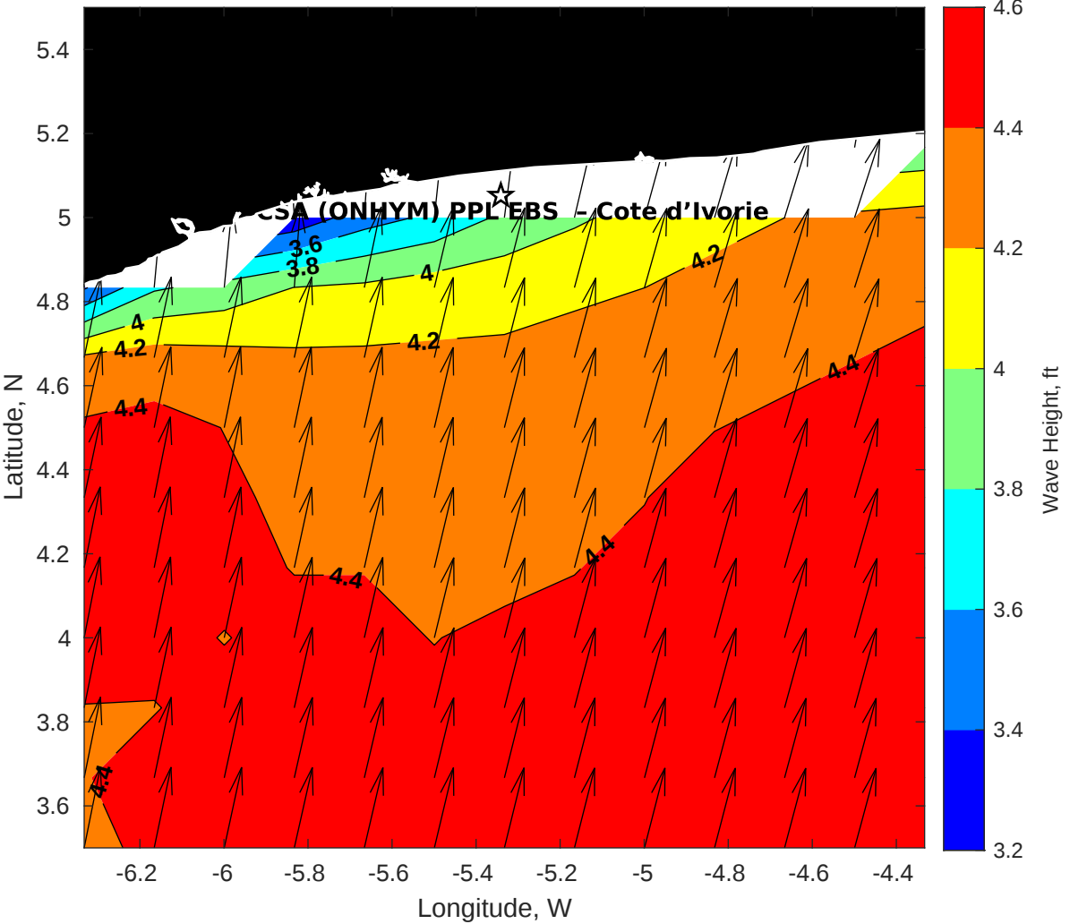
Wave Height (ft) for CSA (ONHYM) PPL EBS - Cote d'Ivoire at 08-Sep-2025 09:00:00
