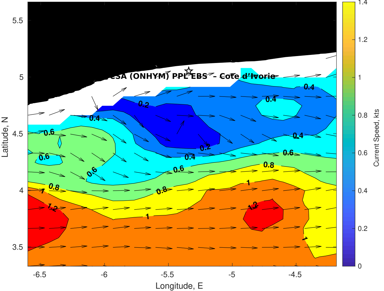
Surface Currents for CSA (ONHYM) PPL EBS - Cote d'Ivoire at 07-Sep-2025 00:00:00
