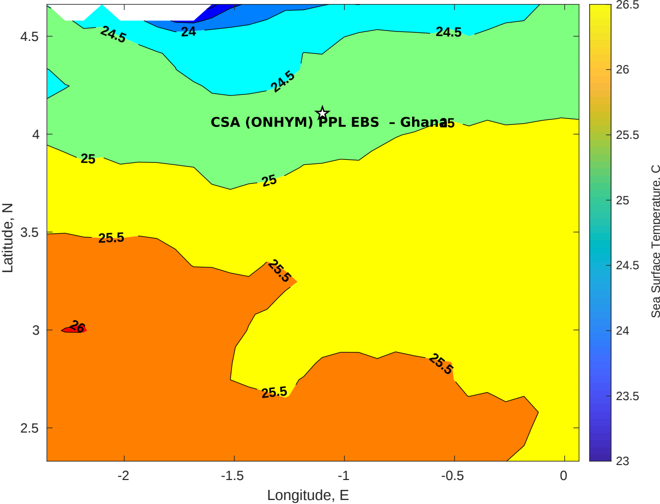
SST for CSA (ONHYM) PPL EBS - Ghana at 07-Sep-2025 00:00:00
