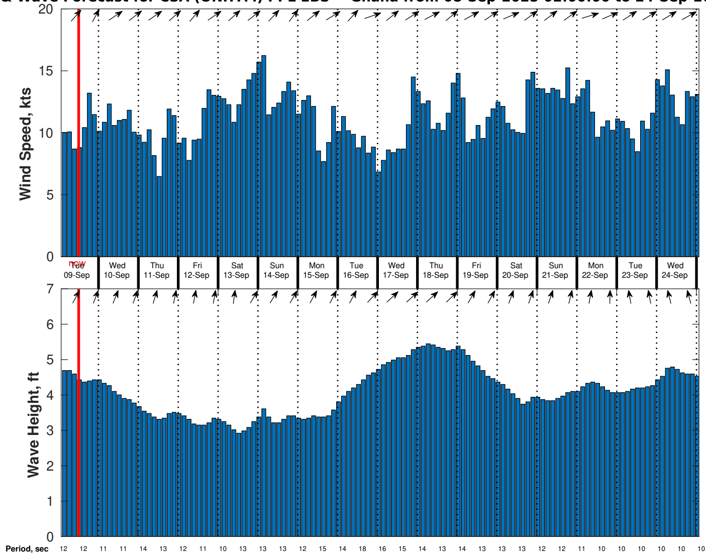
Wind & Wave Forecast for CSA (ONHYM) PPL EBS - Ghana from 08-Sep-2025 02:00:00 to 24-Sep-2025 02:00:00
