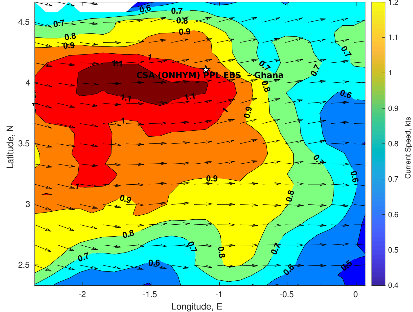
Surface Currents for CSA (ONHYM) PPL EBS - Ghana at 07-Sep-2025 00:00:00
