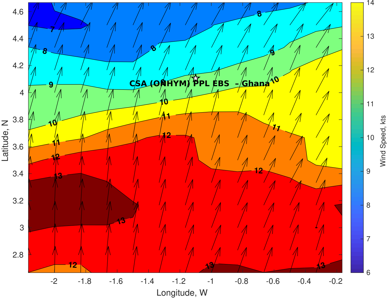
Winds (kts) for CSA (ONHYM) PPL EBS - Ghana at 08-Sep-2025 09:00:00
