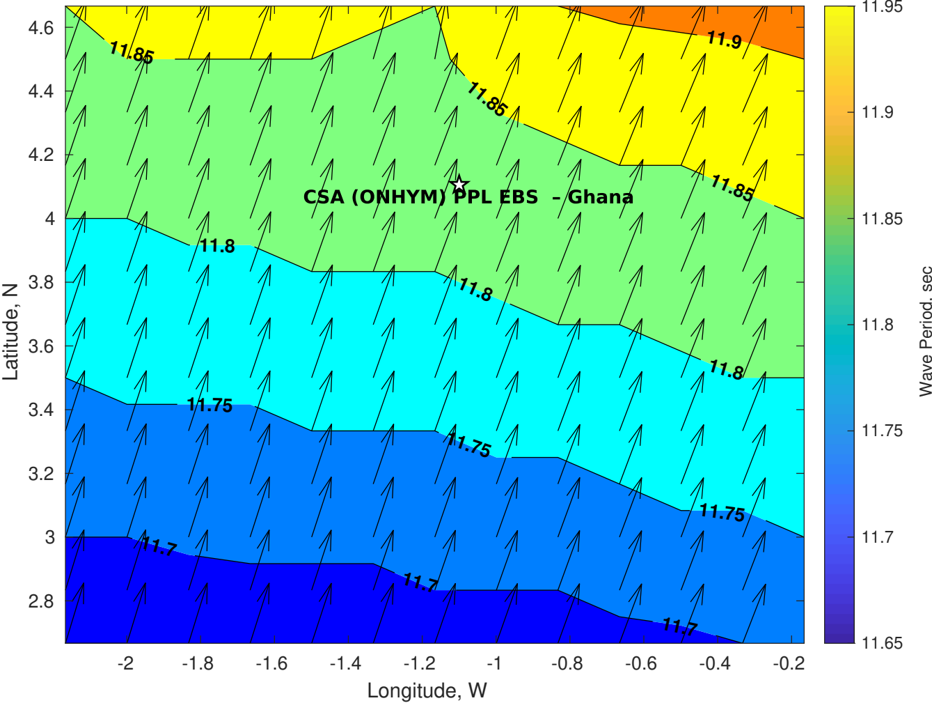
Wave Period (sec) for CSA (ONHYM) PPL EBS - Ghana at 08-Sep-2025 09:00:00
