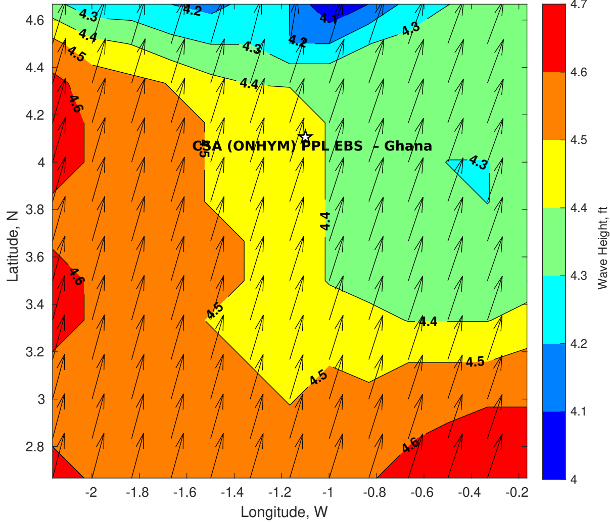
Wave Height (ft) for CSA (ONHYM) PPL EBS - Ghana at 08-Sep-2025 09:00:00
