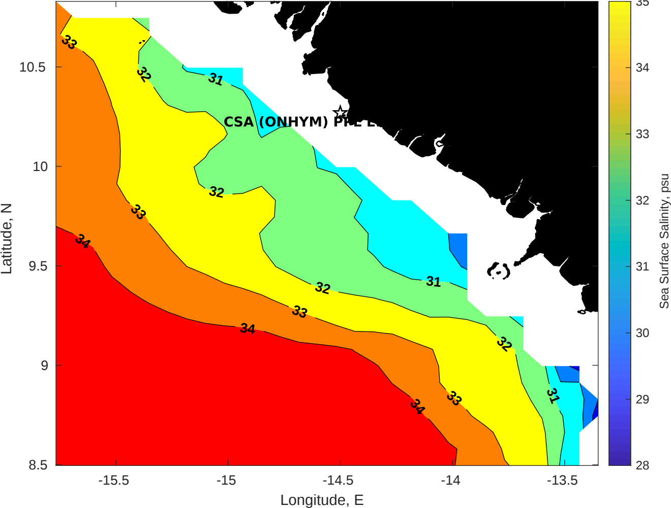
Surface Salinity for CSA (ONHYM) PPL EBS - Guinea at 07-Sep-2025 00:00:00
