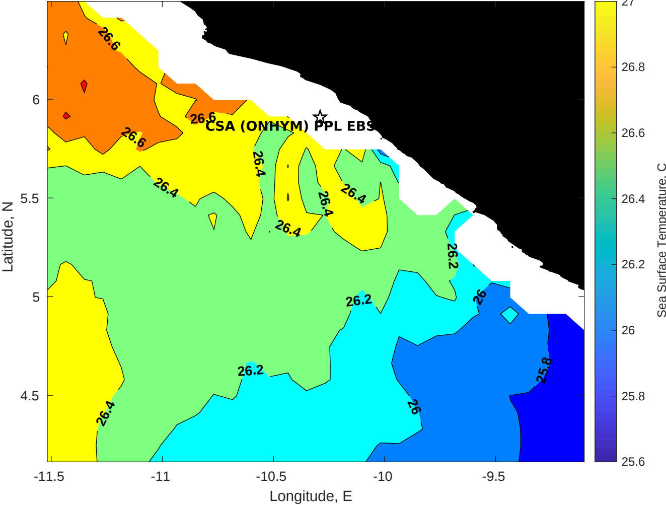
SST for CSA (ONHYM) PPL EBS - Liberia at 07-Sep-2025 00:00:00
