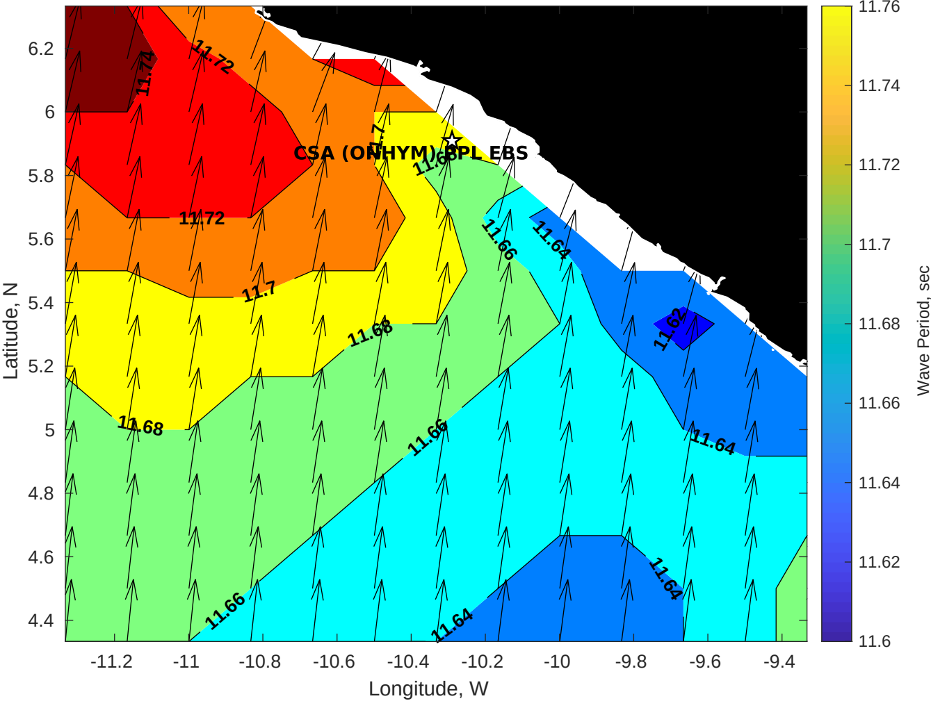
Wave Period (sec) for CSA (ONHYM) PPL EBS - Liberia at 08-Sep-2025 09:00:00
