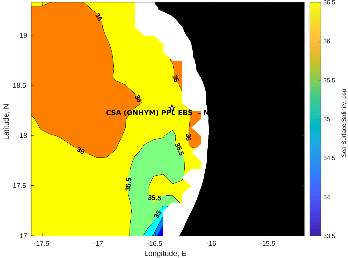
Surface Salinity for CSA (ONHYM) PPL EBS - Mauritania at 07-Sep-2025 00:00:00
