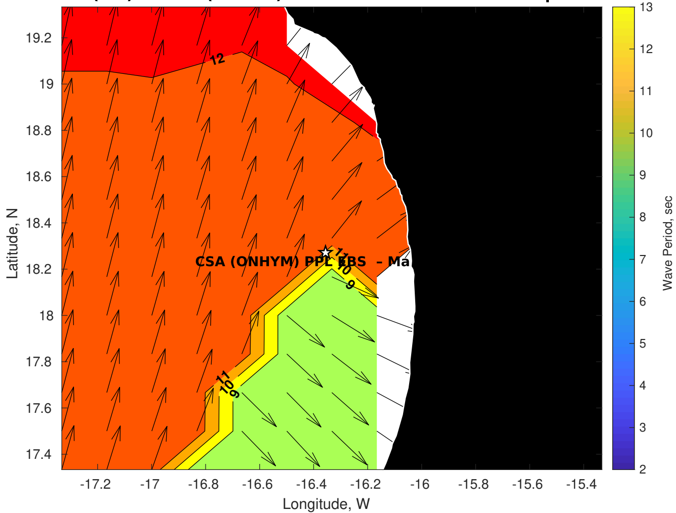
Wave Period (sec) for CSA (ONHYM) PPL EBS - Mauritania at 08-Sep-2025 09:00:00
