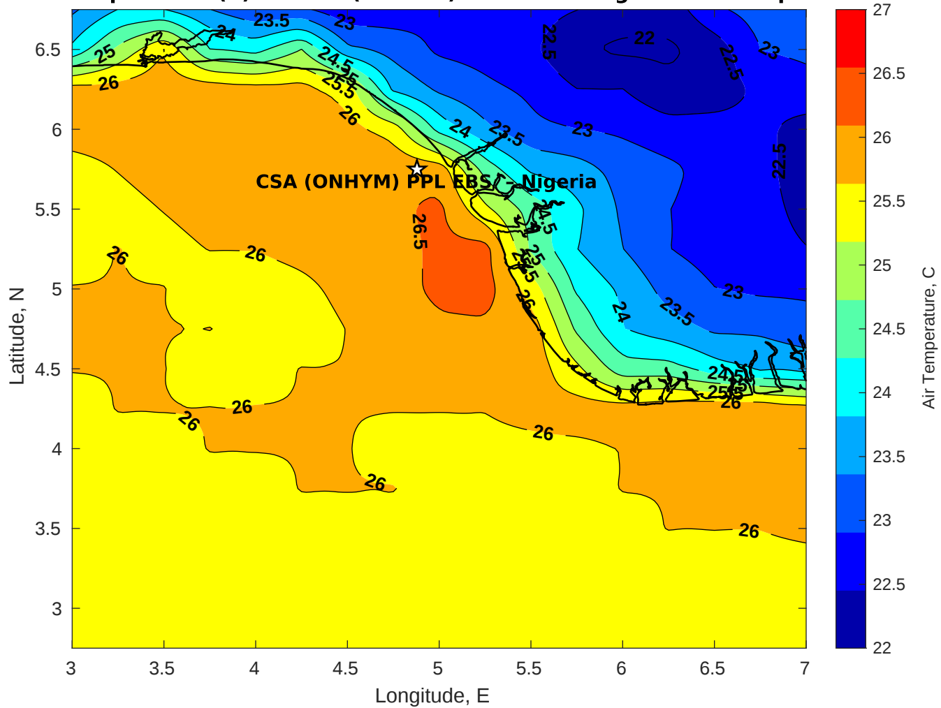
Air Temperature (C) for CSA (ONHYM) PPL EBS - Nigeria at 08-Sep-2025
