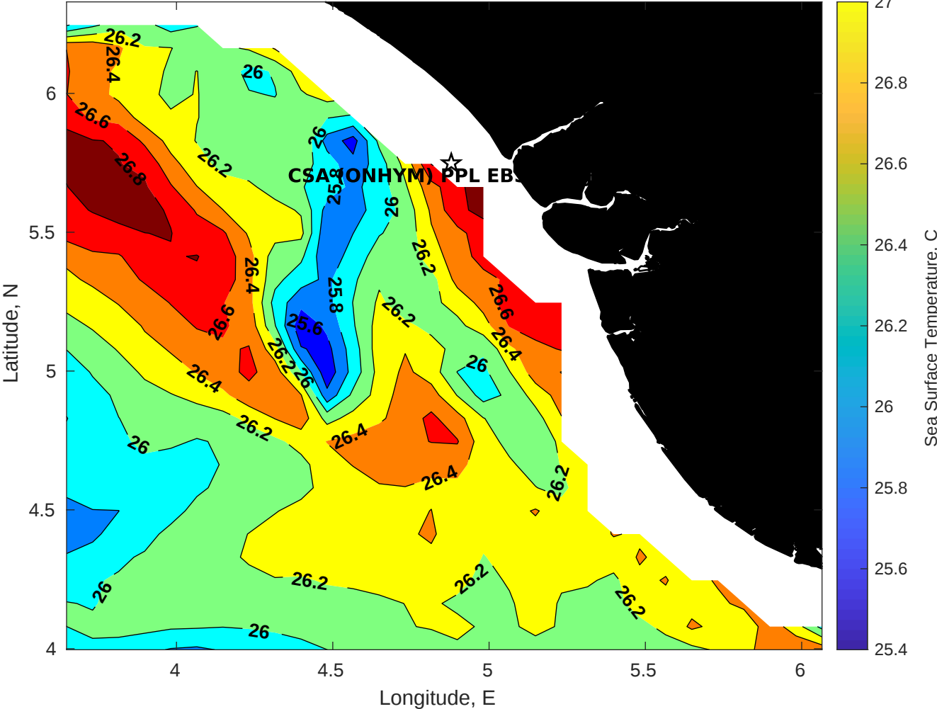
SST for CSA (ONHYM) PPL EBS - Nigeria at 07-Sep-2025 00:00:00
