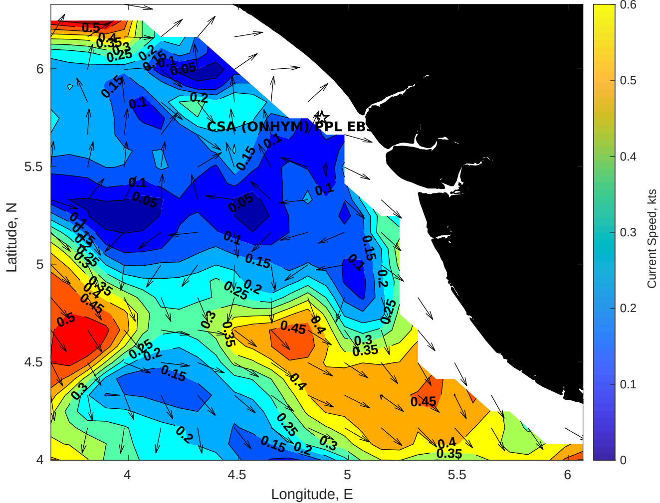
Surface Currents for CSA (ONHYM) PPL EBS - Nigeria at 07-Sep-2025 00:00:00
