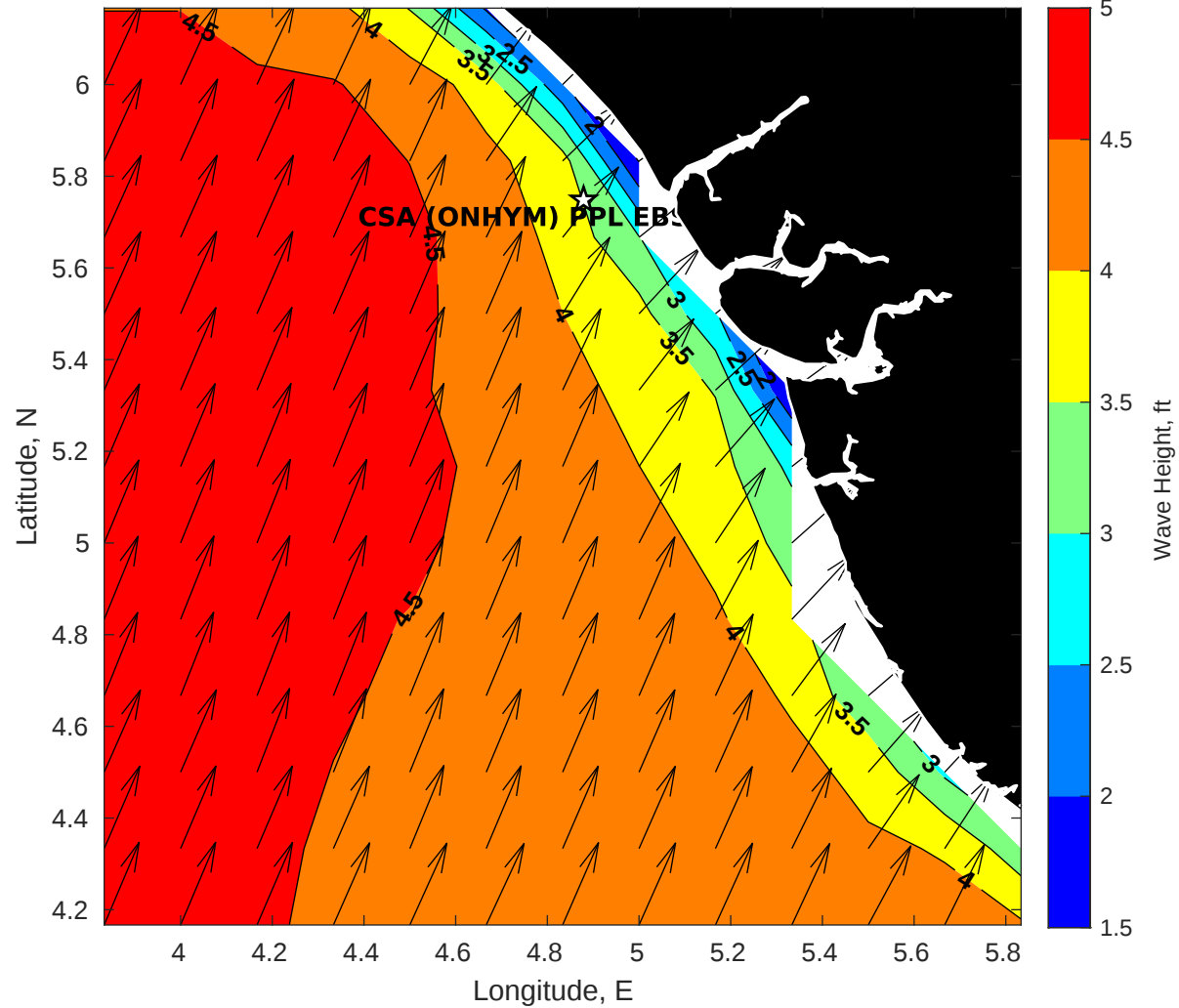
Wave Height (ft) for CSA (ONHYM) PPL EBS - Nigeria at 08-Sep-2025 09:00:00
