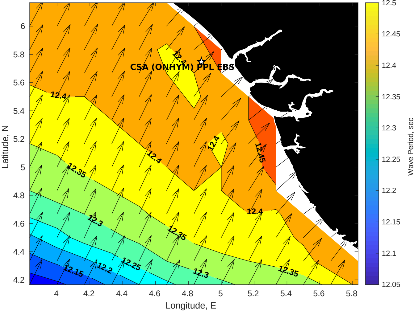
Wave Period (sec) for CSA (ONHYM) PPL EBS - Nigeria at 08-Sep-2025 09:00:00
