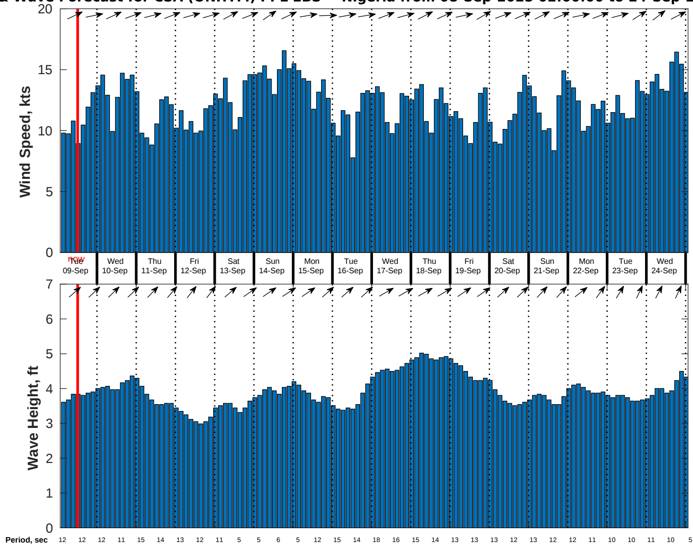
Wind & Wave Forecast for CSA (ONHYM) PPL EBS - Nigeria from 08-Sep-2025 02:00:00 to 24-Sep-2025 02:00:00
