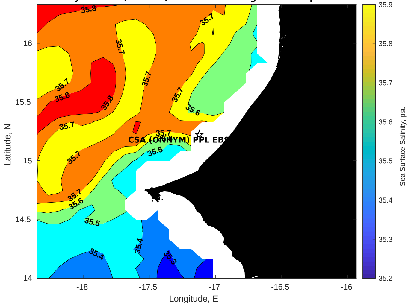
Surface Salinity for CSA (ONHYM) PPL EBS - Senegal at 07-Sep-2025 00:00:00
