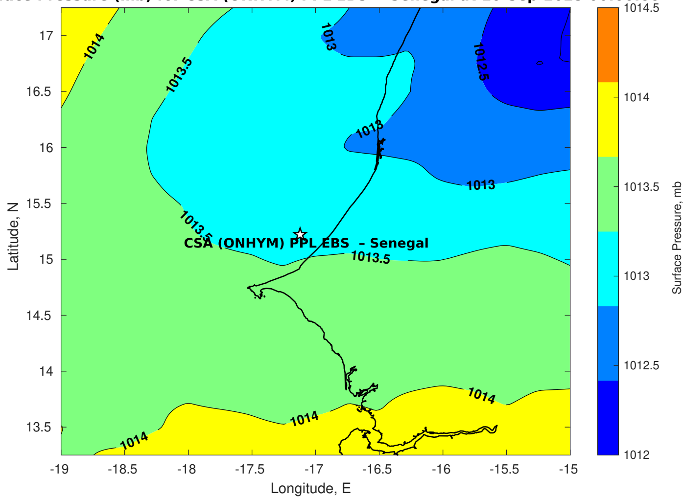
Surface Pressure (mb) for CSA (ONHYM) PPL EBS - Senegal at 10-Sep-2025 00:00:00
