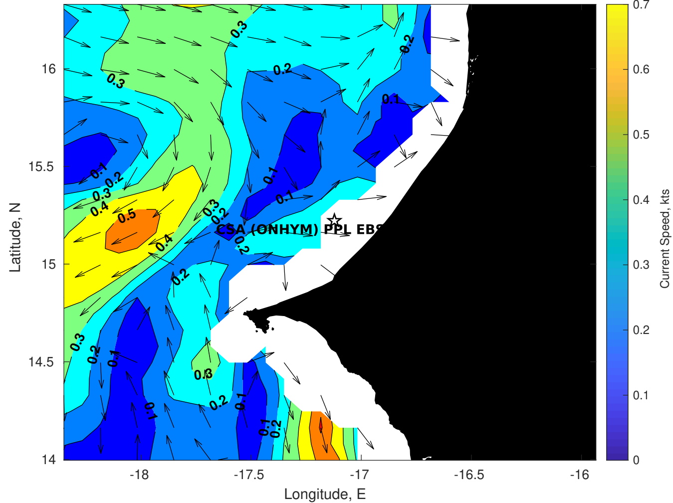
Surface Currents for CSA (ONHYM) PPL EBS - Senegal at 07-Sep-2025 00:00:00
