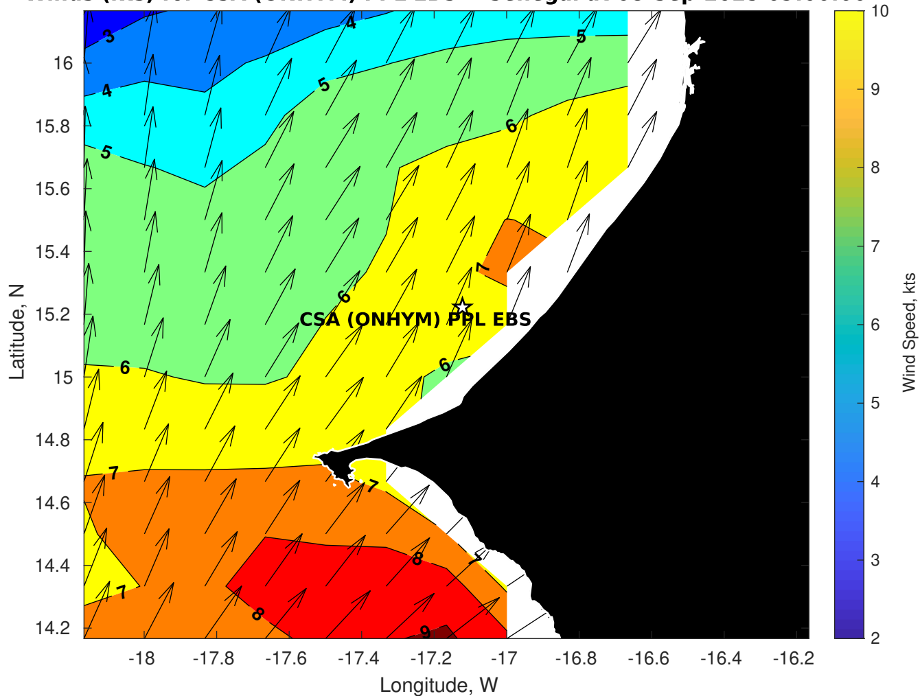
Winds (kts) for CSA (ONHYM) PPL EBS - Senegal at 08-Sep-2025 09:00:00
