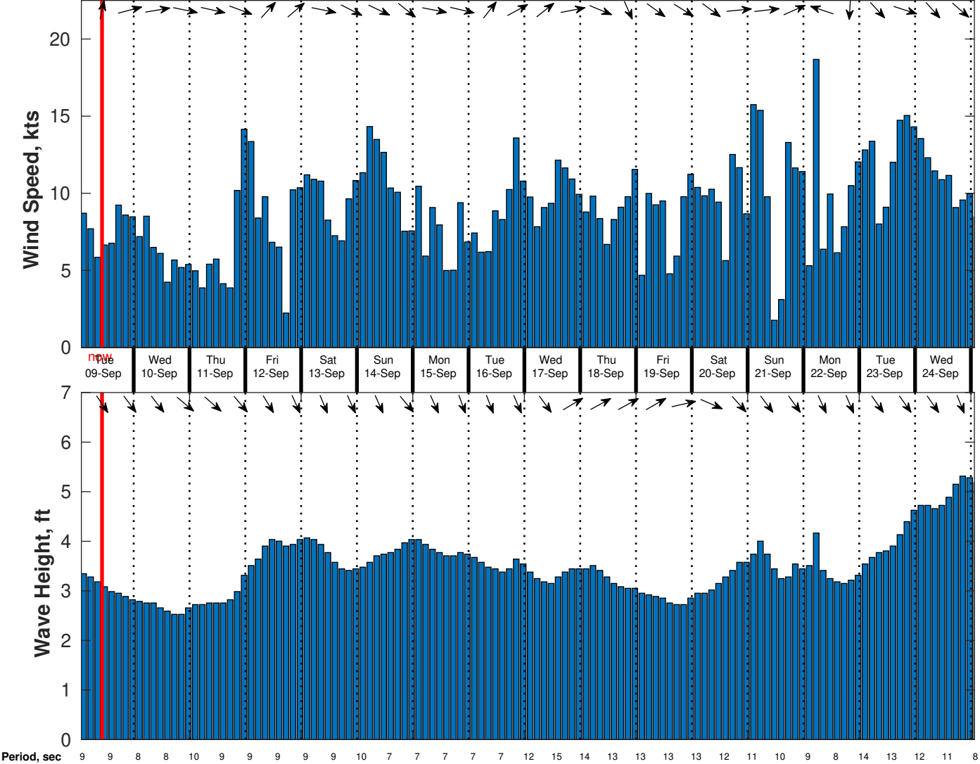
Wind & Wave Forecast for CSA (ONHYM) PPL EBS - Senegal from 08-Sep-2025 01:00:00 to 24-Sep-2025 01:00:00
