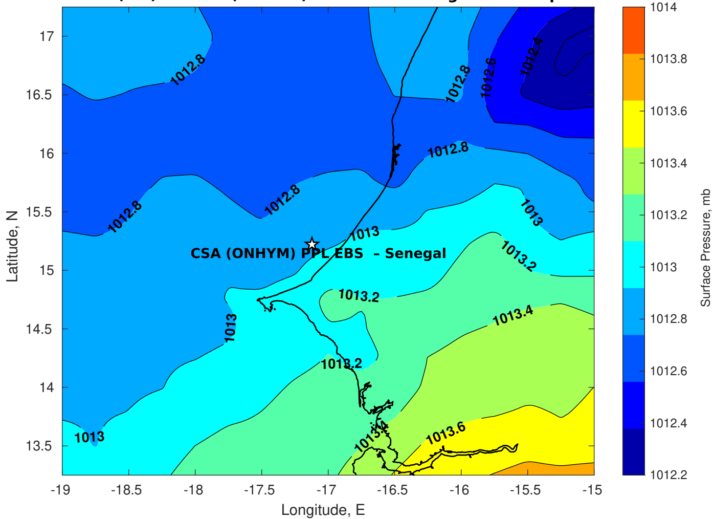
Surface Pressure (mb) for CSA (ONHYM) PPL EBS - Senegal at 08-Sep-2025 00:00:00
