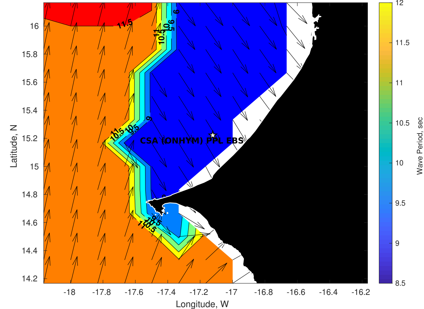
Wave Period (sec) for CSA (ONHYM) PPL EBS - Senegal at 08-Sep-2025 09:00:00
