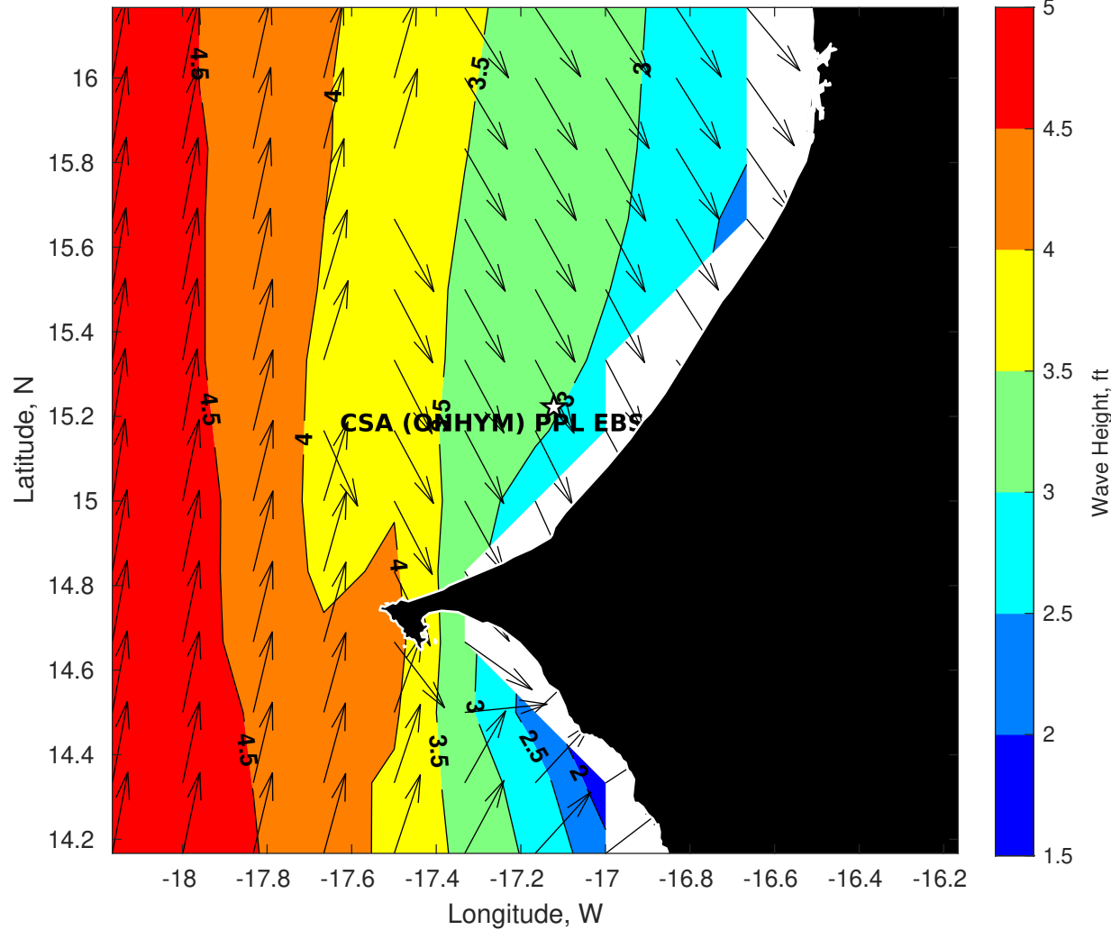
Wave Height (ft) for CSA (ONHYM) PPL EBS - Senegal at 08-Sep-2025 09:00:00
