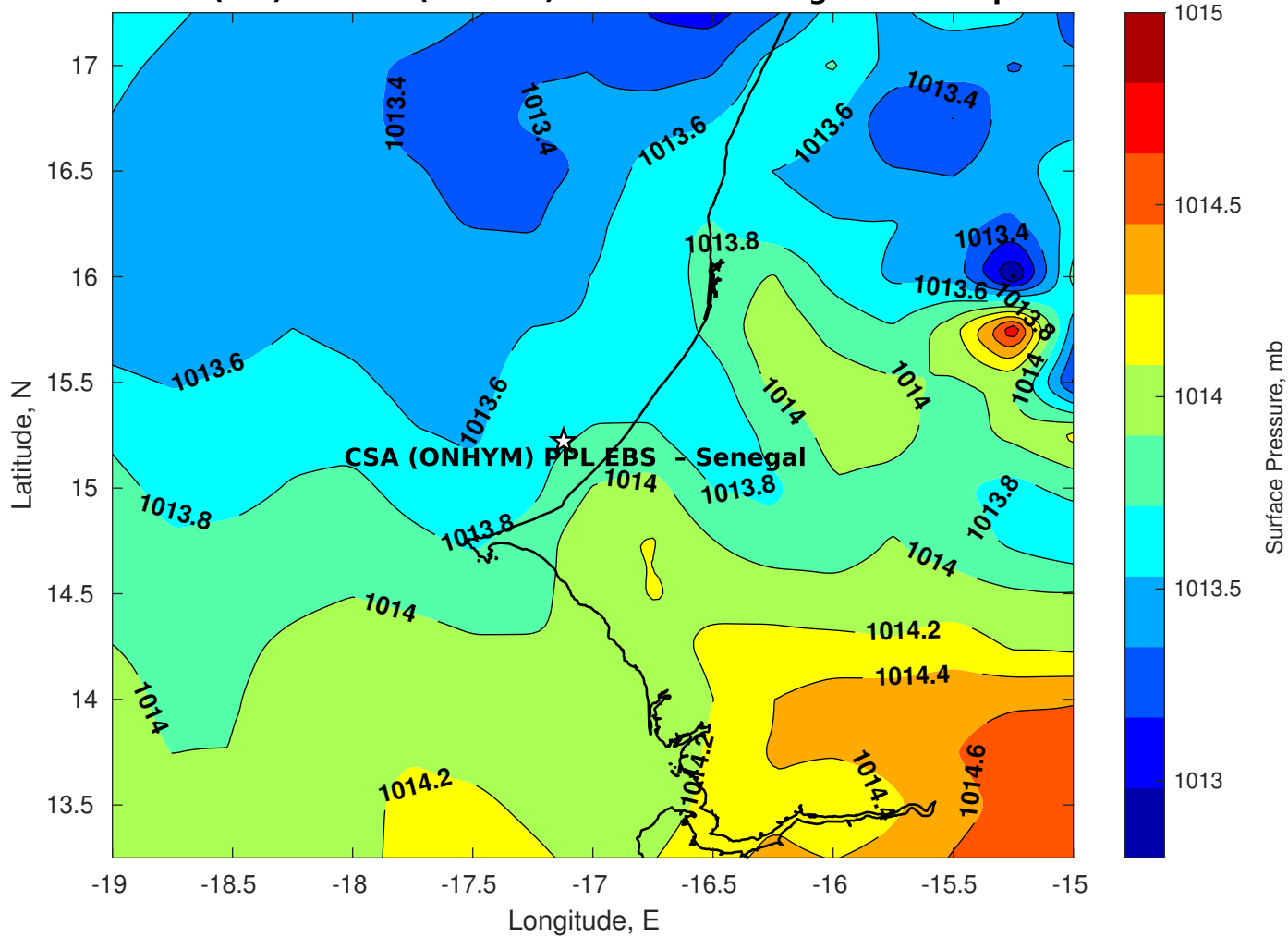
Surface Pressure (mb) for CSA (ONHYM) PPL EBS - Senegal at 09-Sep-2025 00:00:00
