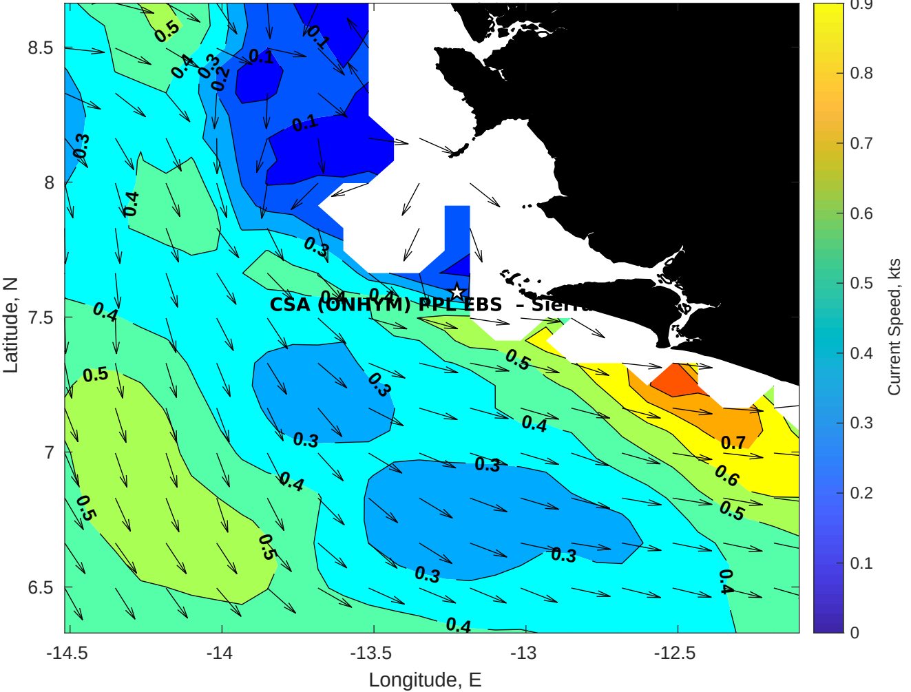
Surface Currents for CSA (ONHYM) PPL EBS - Sierra Leone at 07-Sep-2025 00:00:00
