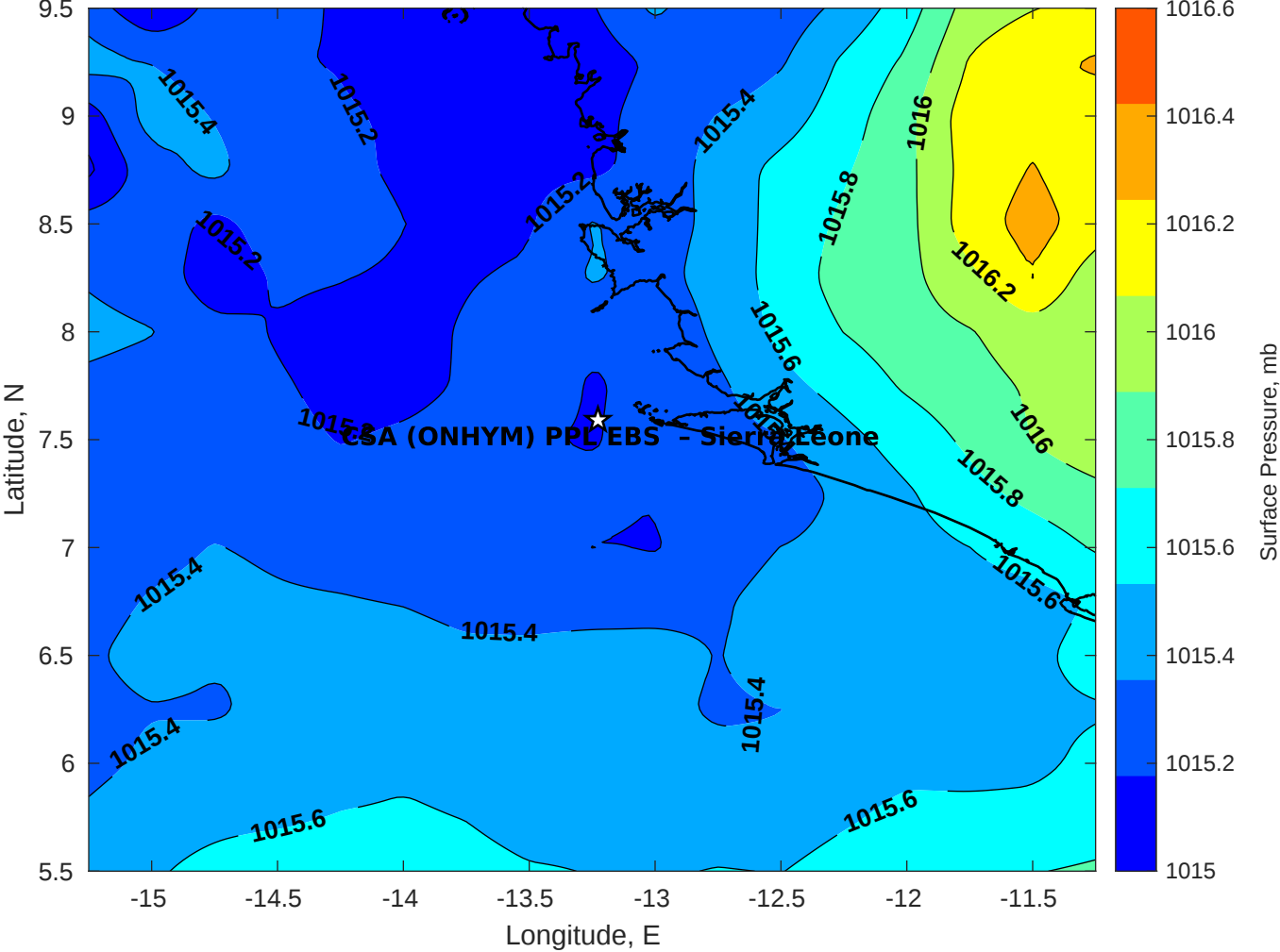
Surface Pressure (mb) for CSA (ONHYM) PPL EBS - Sierra Leone at 10-Sep-2025 00:00:00
