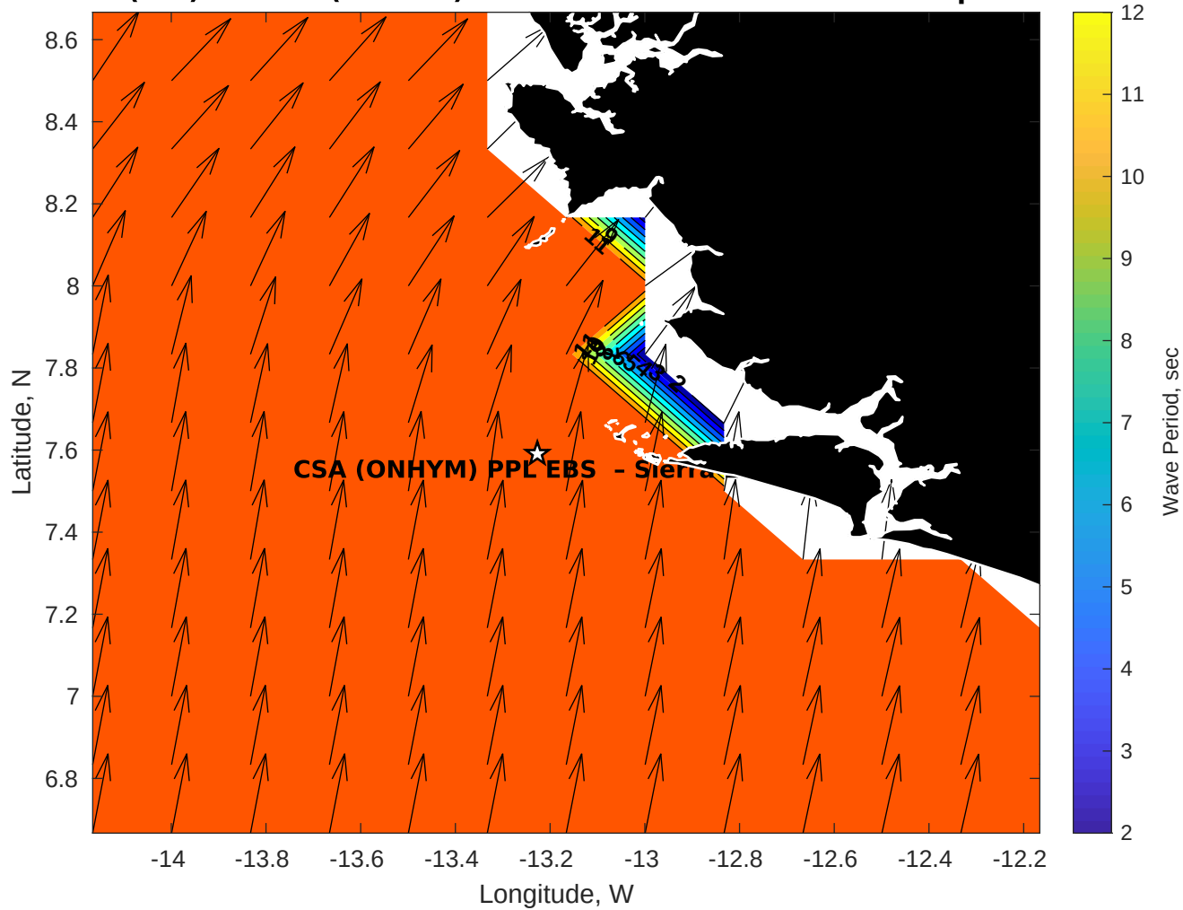
Wave Period (sec) for CSA (ONHYM) PPL EBS - Sierra Leone at 08-Sep-2025 09:00:00
