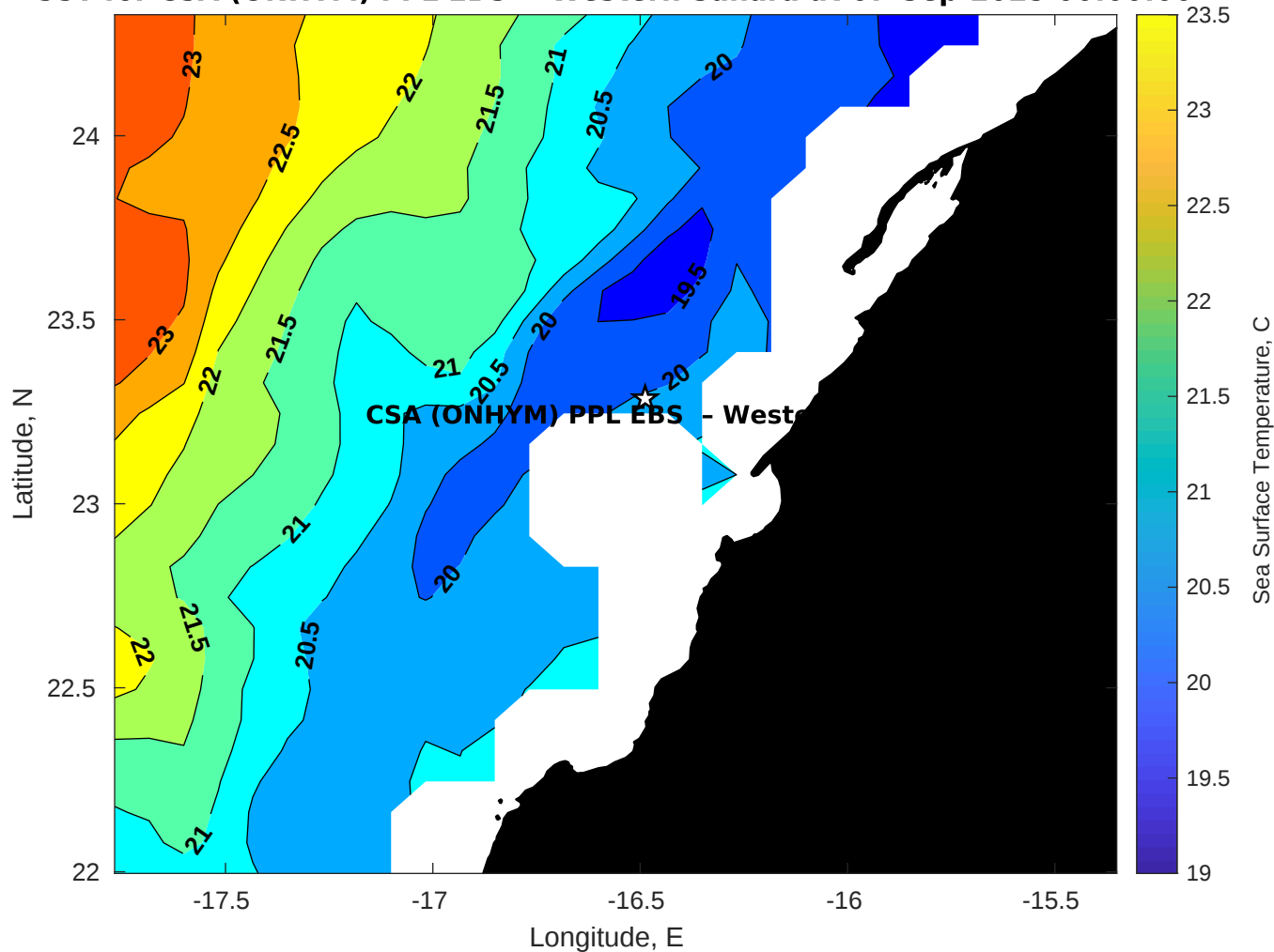
SST for CSA (ONHYM) PPL EBS - Western Sahara at 07-Sep-2025 00:00:00
