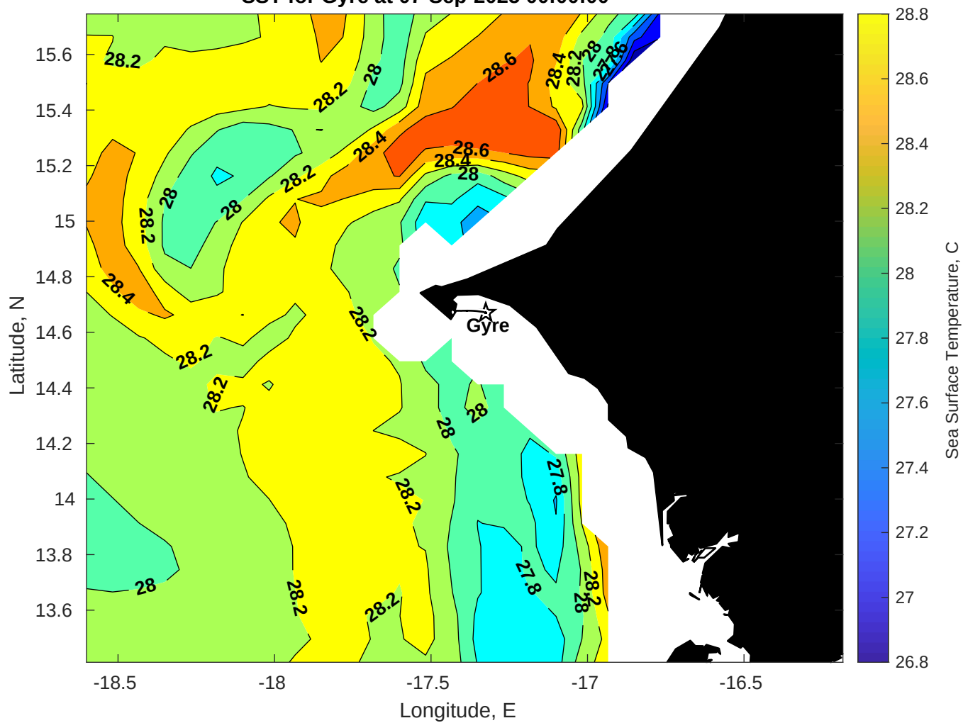
SST for Gyre at 07-Sep-2025 00:00:00
