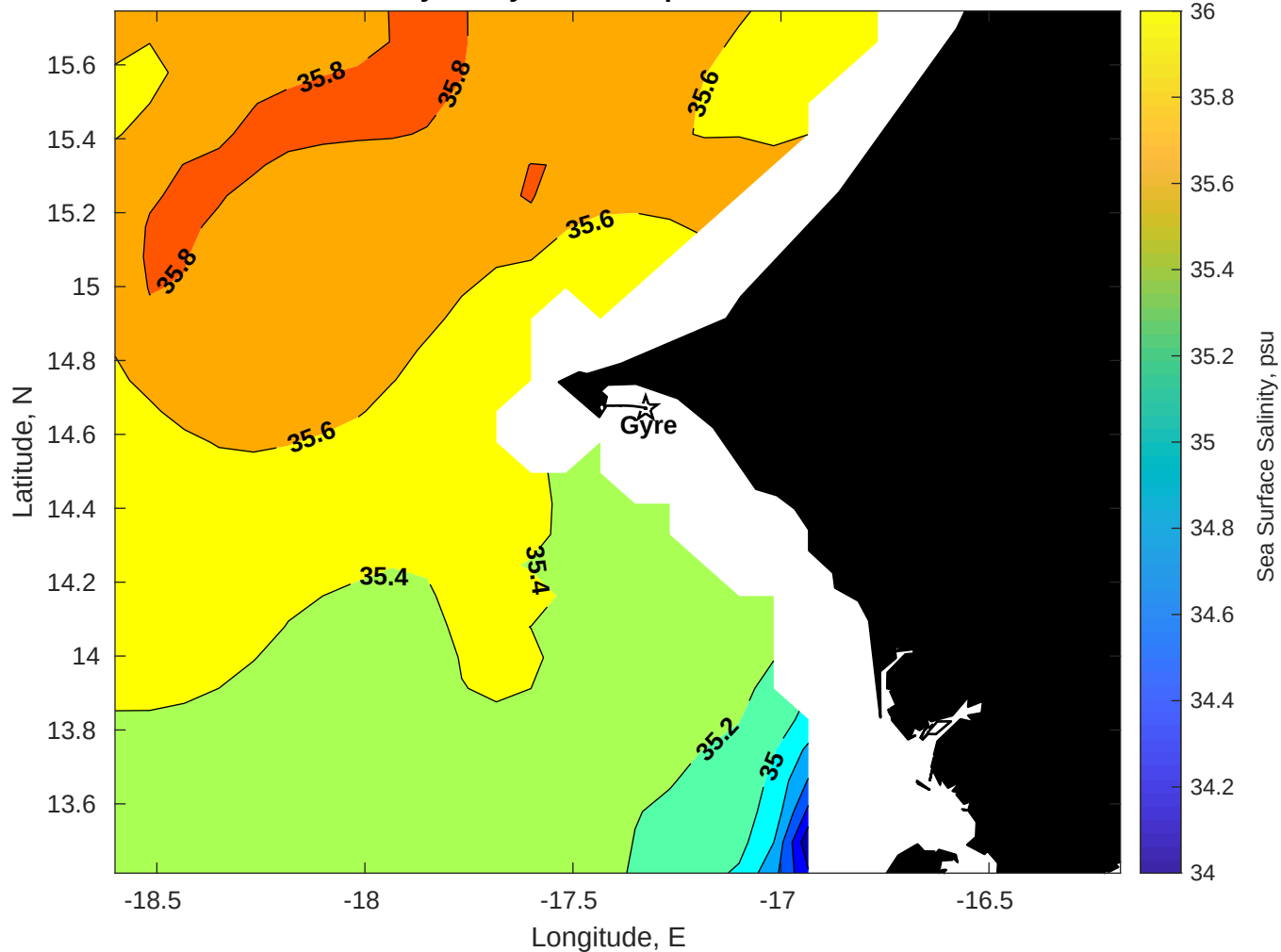
Surface Salinity for Gyre at 07-Sep-2025 00:00:00
