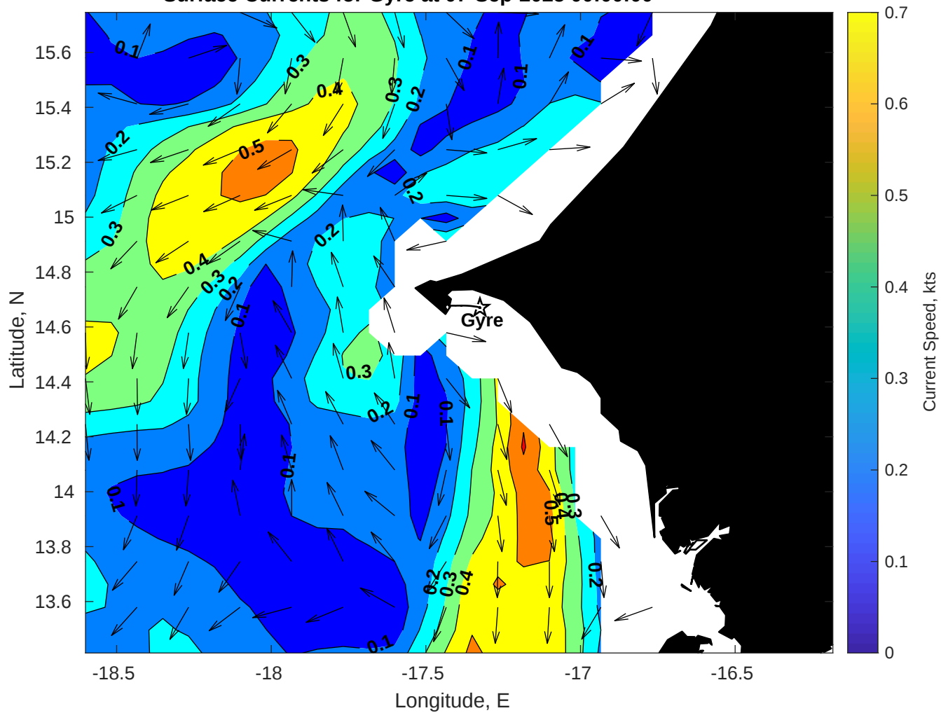
Surface Currents for Gyre at 07-Sep-2025 00:00:00
