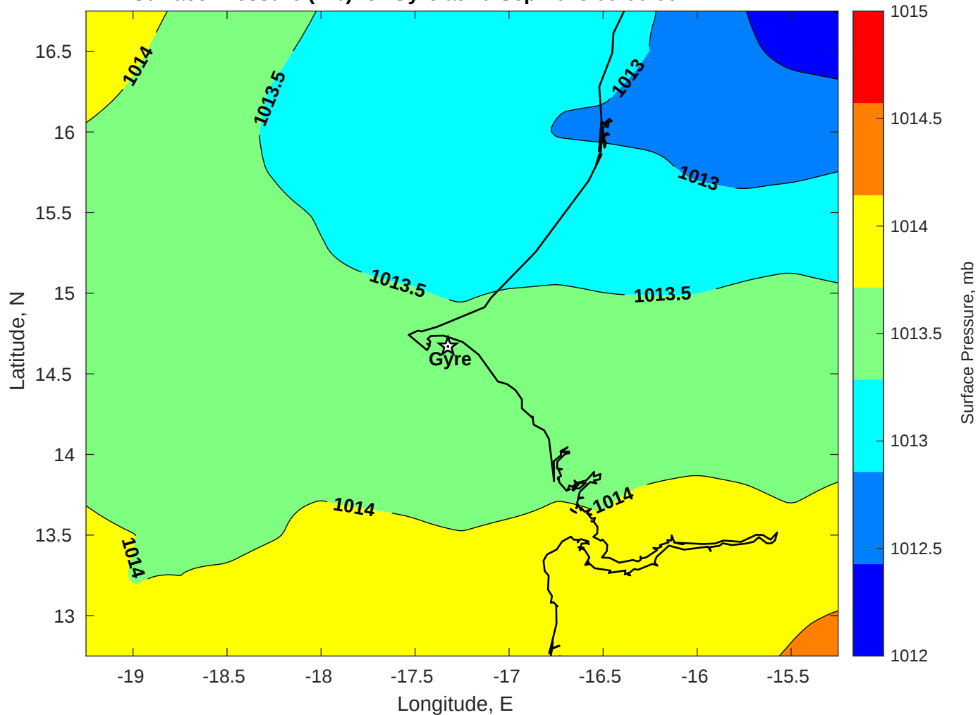
Surface Pressure (mb) for Gyre at 10-Sep-2025 00:00:00
