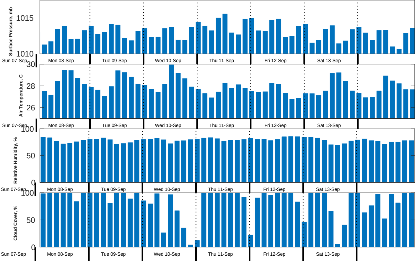
Met Forecast for Gyre from 07-Sep-2025 23:00:00 to 14-Sep-2025 23:00:00
