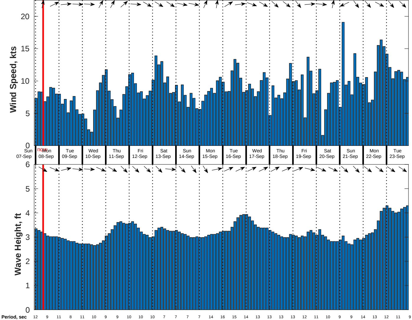
Wind & Wave Forecast for Gyre from 07-Sep-2025 23:00:00 to 23-Sep-2025 23:00:00
