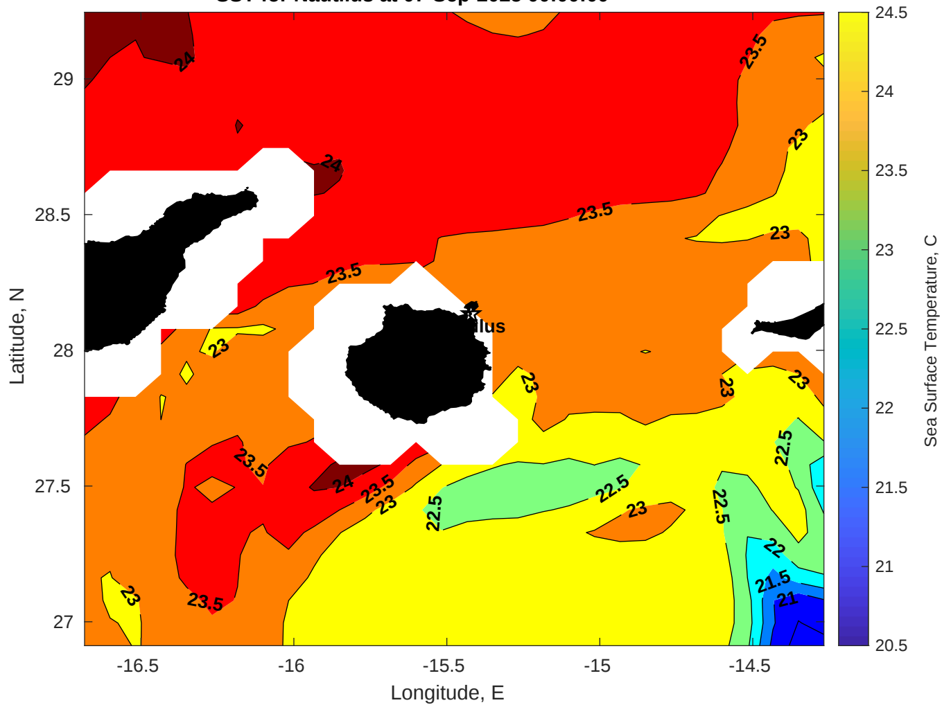
SST for Nautilus at 07-Sep-2025 00:00:00
