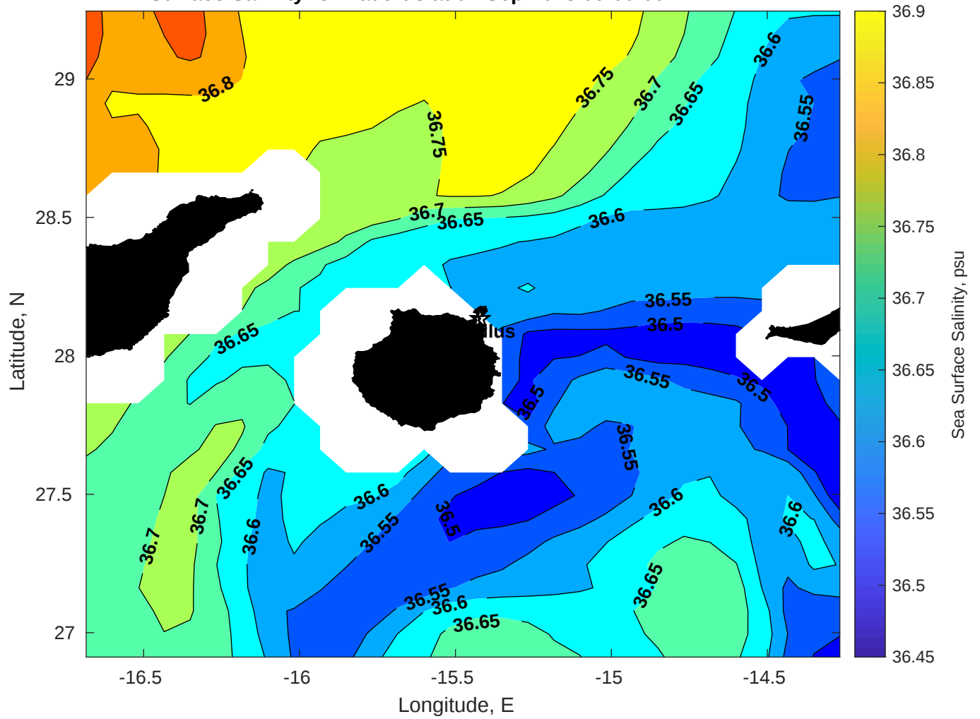
Surface Salinity for Nautilus at 07-Sep-2025 00:00:00
