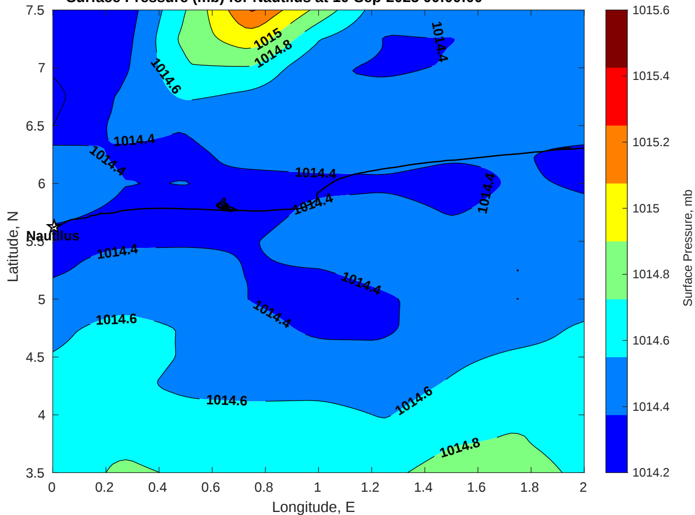
Surface Pressure (mb) for Nautilus at 10-Sep-2025 00:00:00
