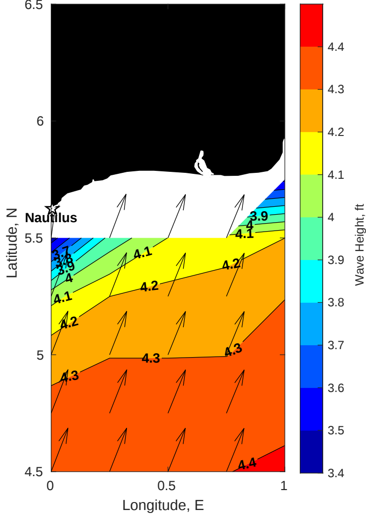
Wave Height (ft) for Nautilus at 08-Sep-2025 09:00:00
