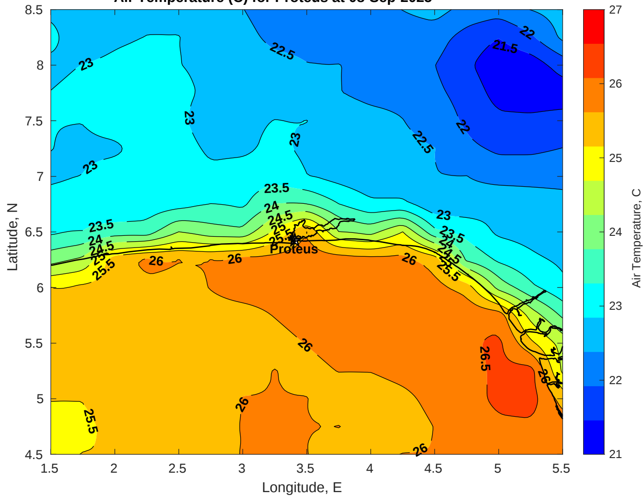
Air Temperature (C) for Proteus at 08-Sep-2025
