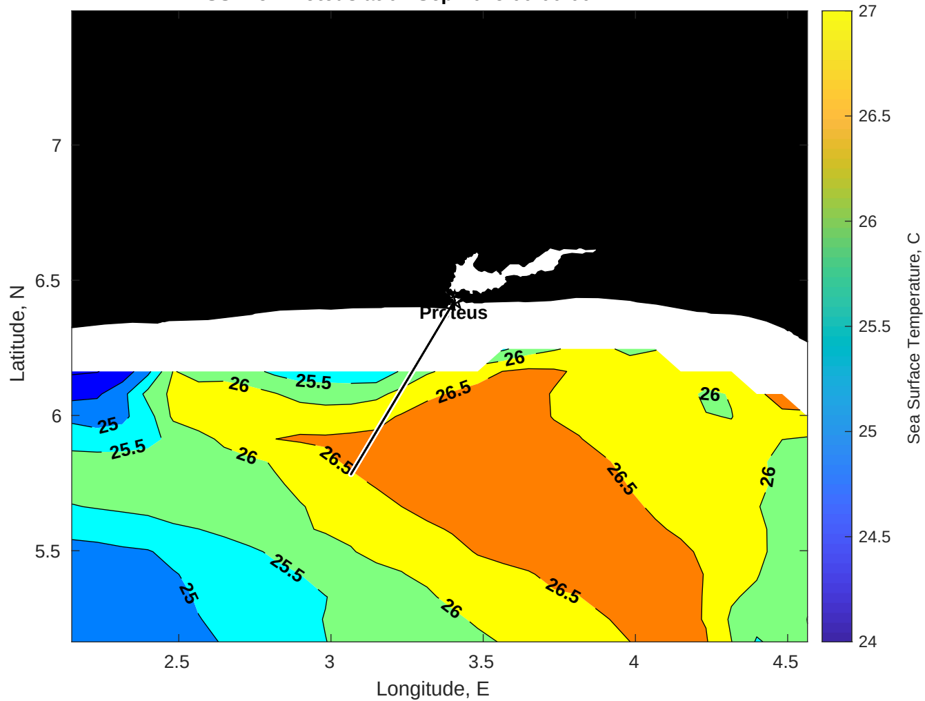
SST for Proteus at 07-Sep-2025 00:00:00
