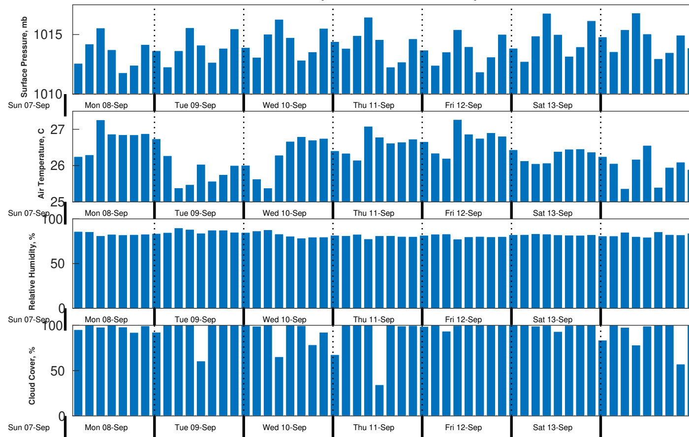
Met Forecast for Proteus from 08-Sep-2025 00:00:00 to 15-Sep-2025 00:00:00
