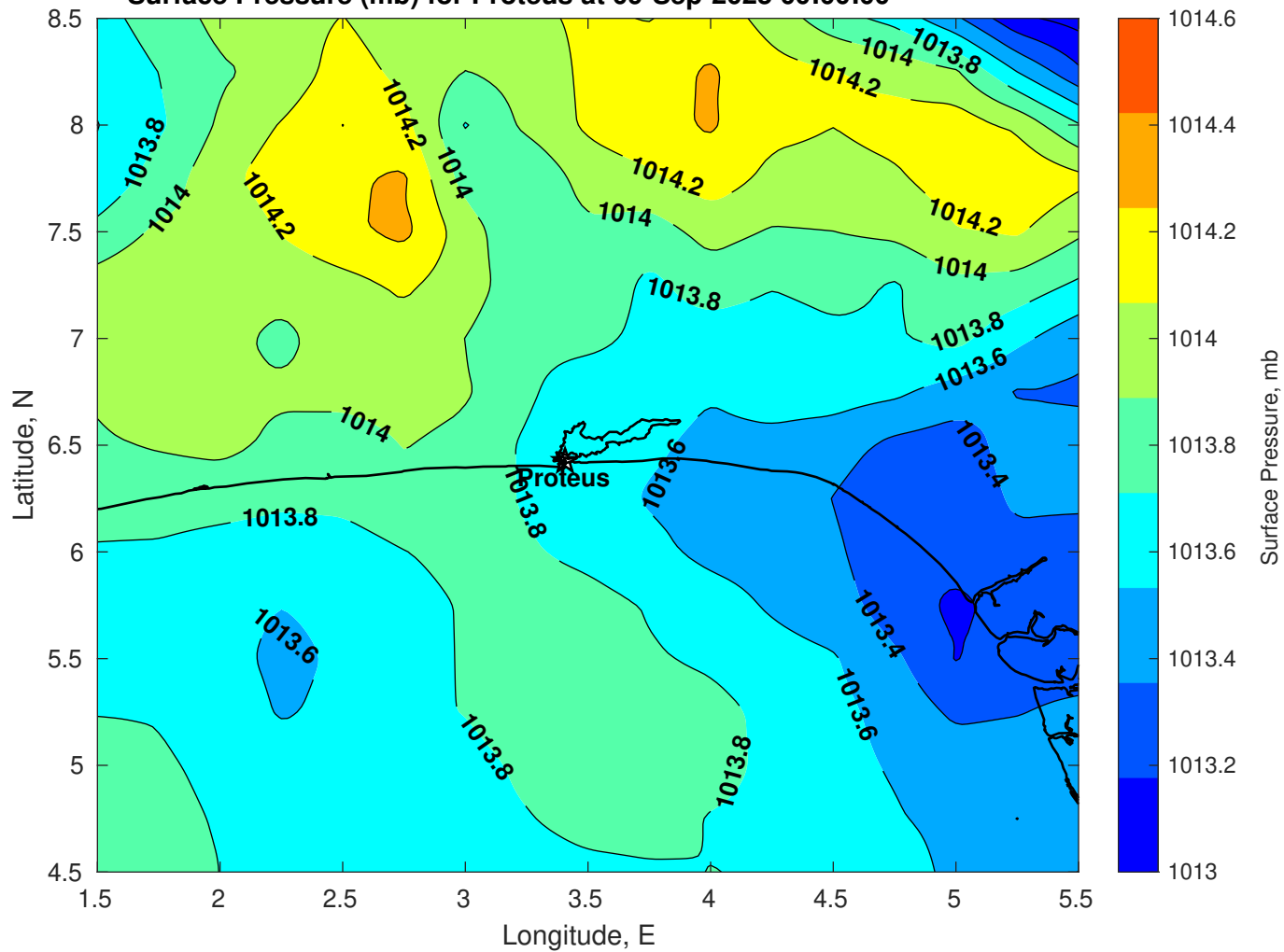
Surface Pressure (mb) for Proteus at 09-Sep-2025 00:00:00
