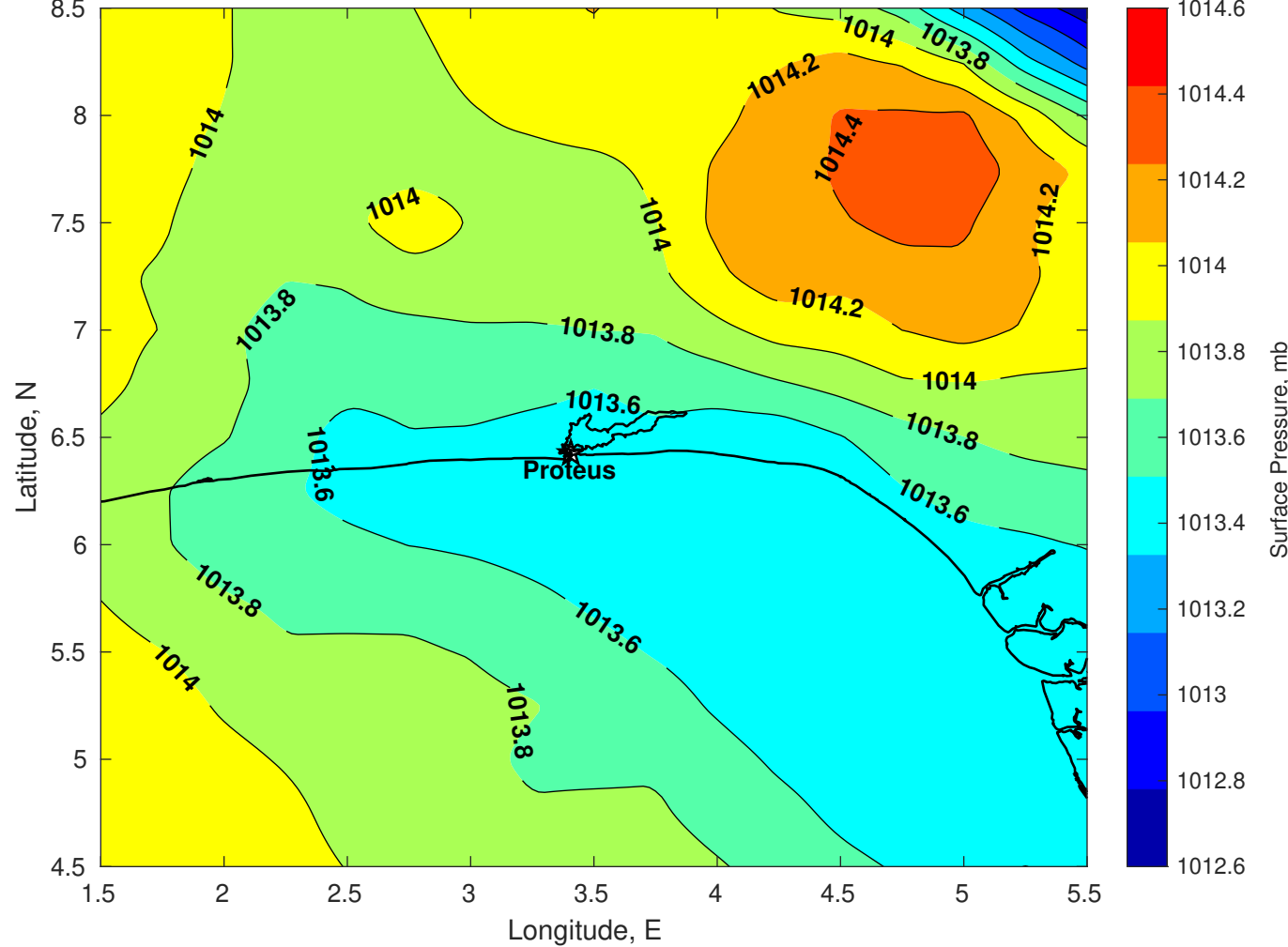
Surface Pressure (mb) for Proteus at 08-Sep-2025 00:00:00
