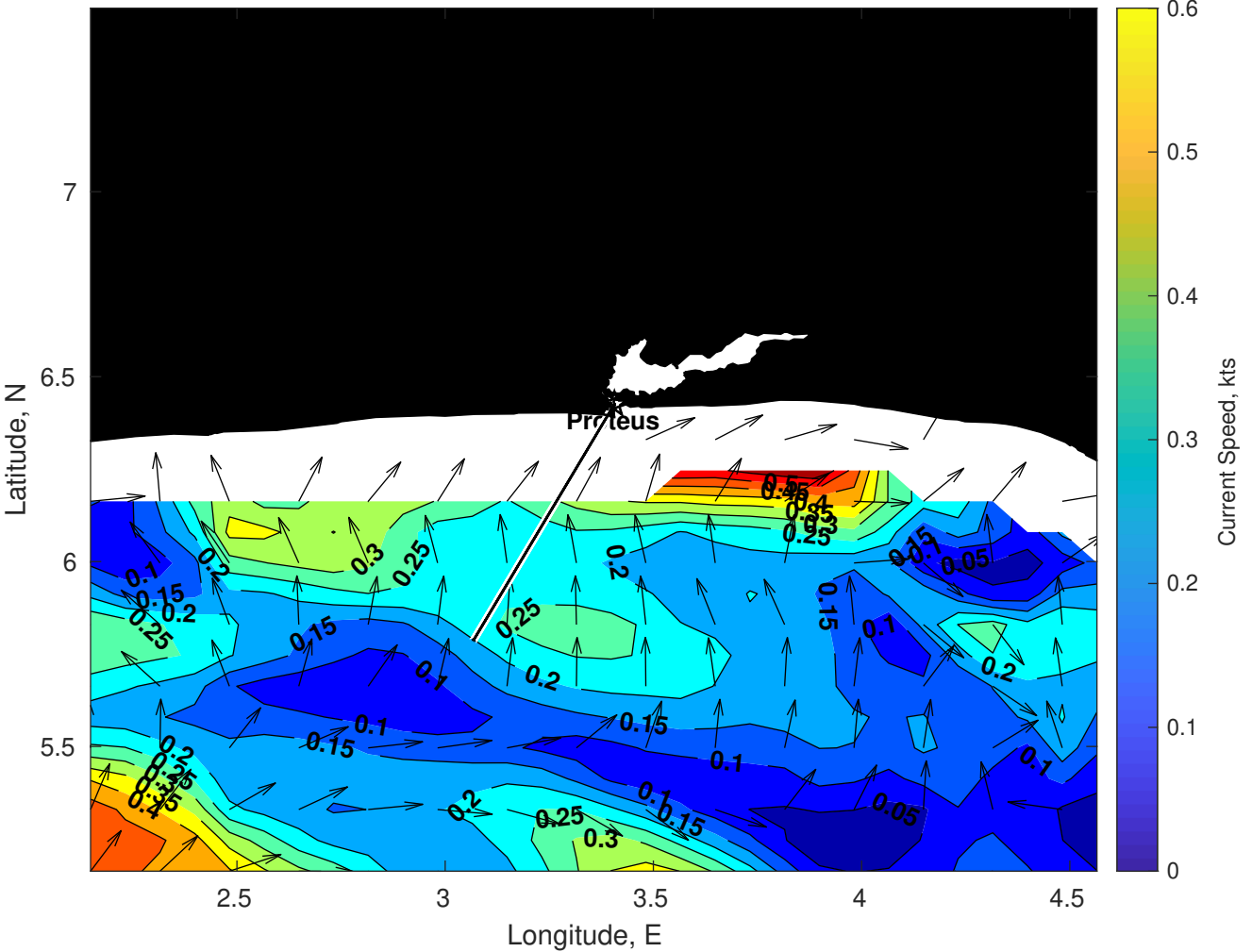
Surface Currents for Proteus at 07-Sep-2025 00:00:00
