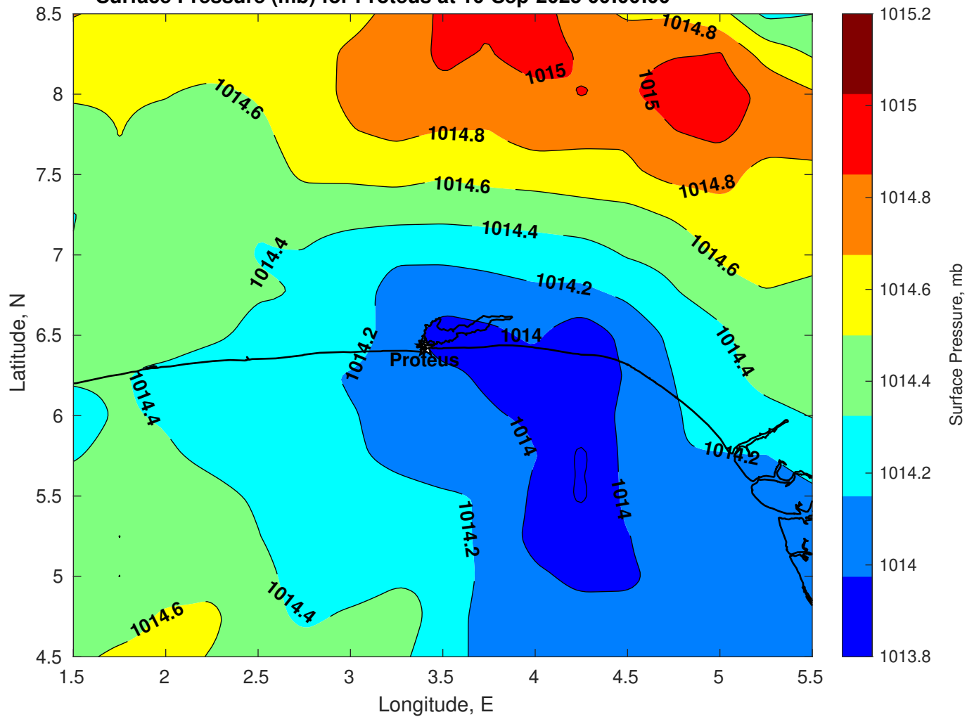
Surface Pressure (mb) for Proteus at 10-Sep-2025 00:00:00
