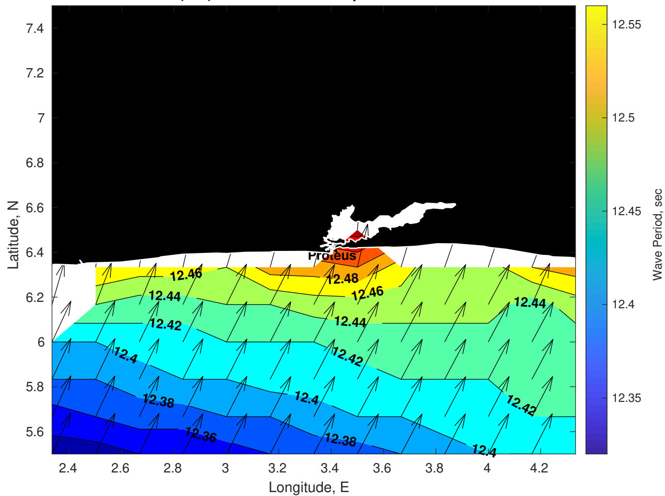
Wave Period (sec) for Proteus at 08-Sep-2025 09:00:00
