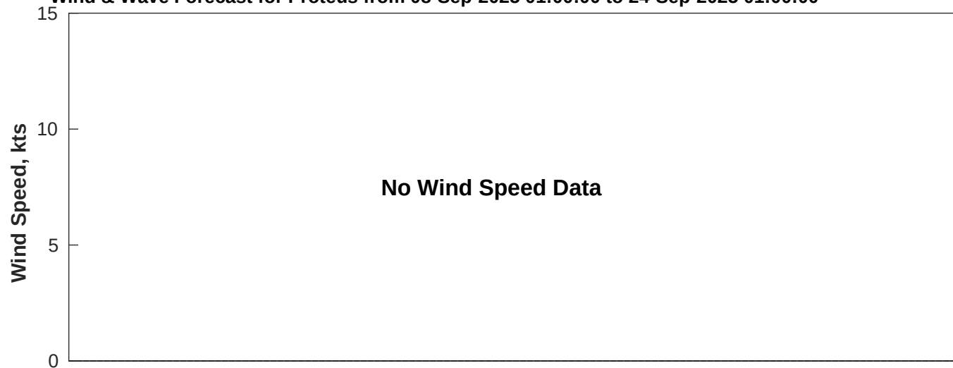
Wind & Wave Forecast for Proteus from 08-Sep-2025 01:00:00 to 24-Sep-2025 01:00:00
