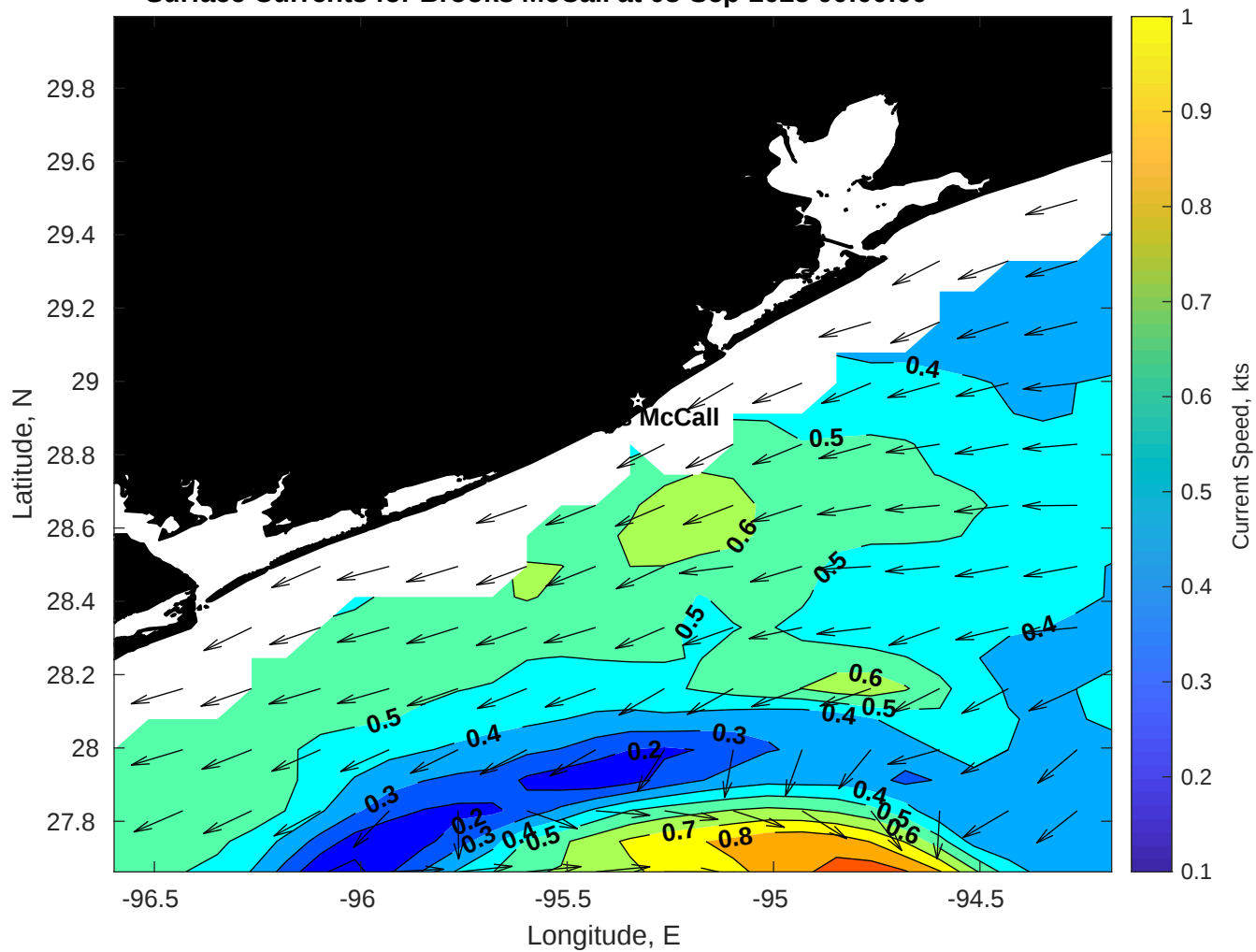
Surface Currents for Brooks McCall at 08-Sep-2025 00:00:00
